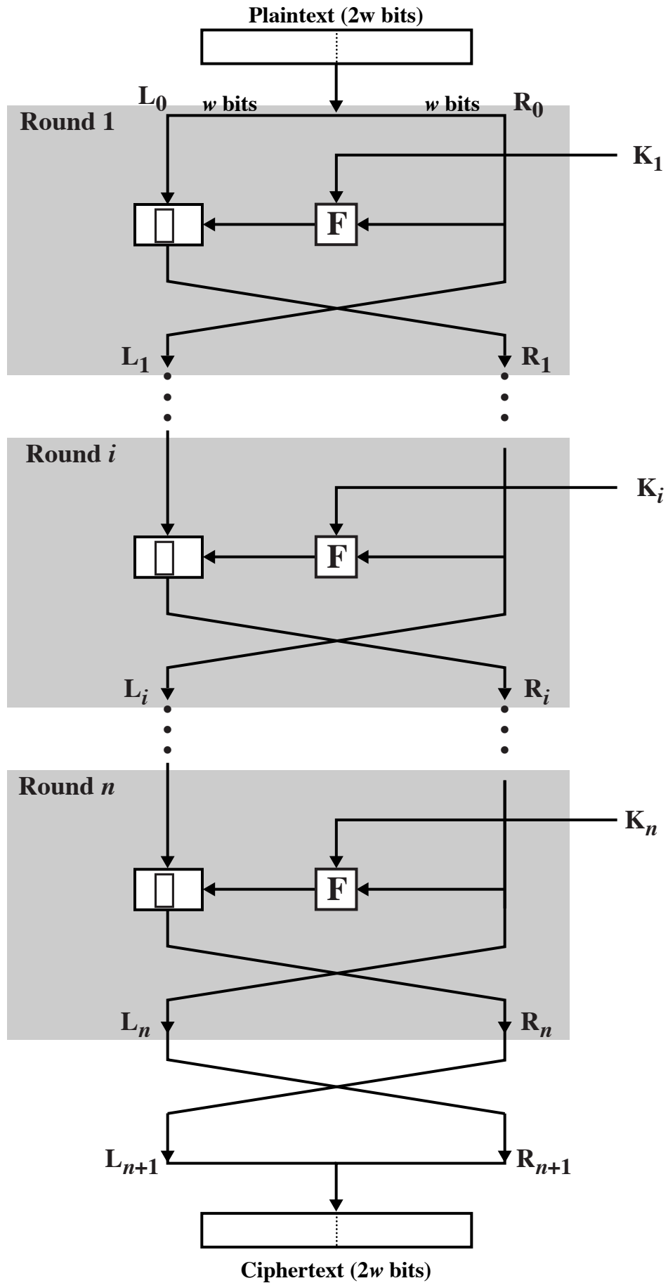
Figure 3.5 Classical Feistel Network
