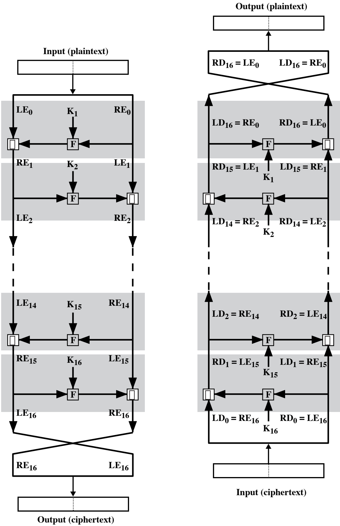
Figure 3.6 Feistel Encryption and Decryption
