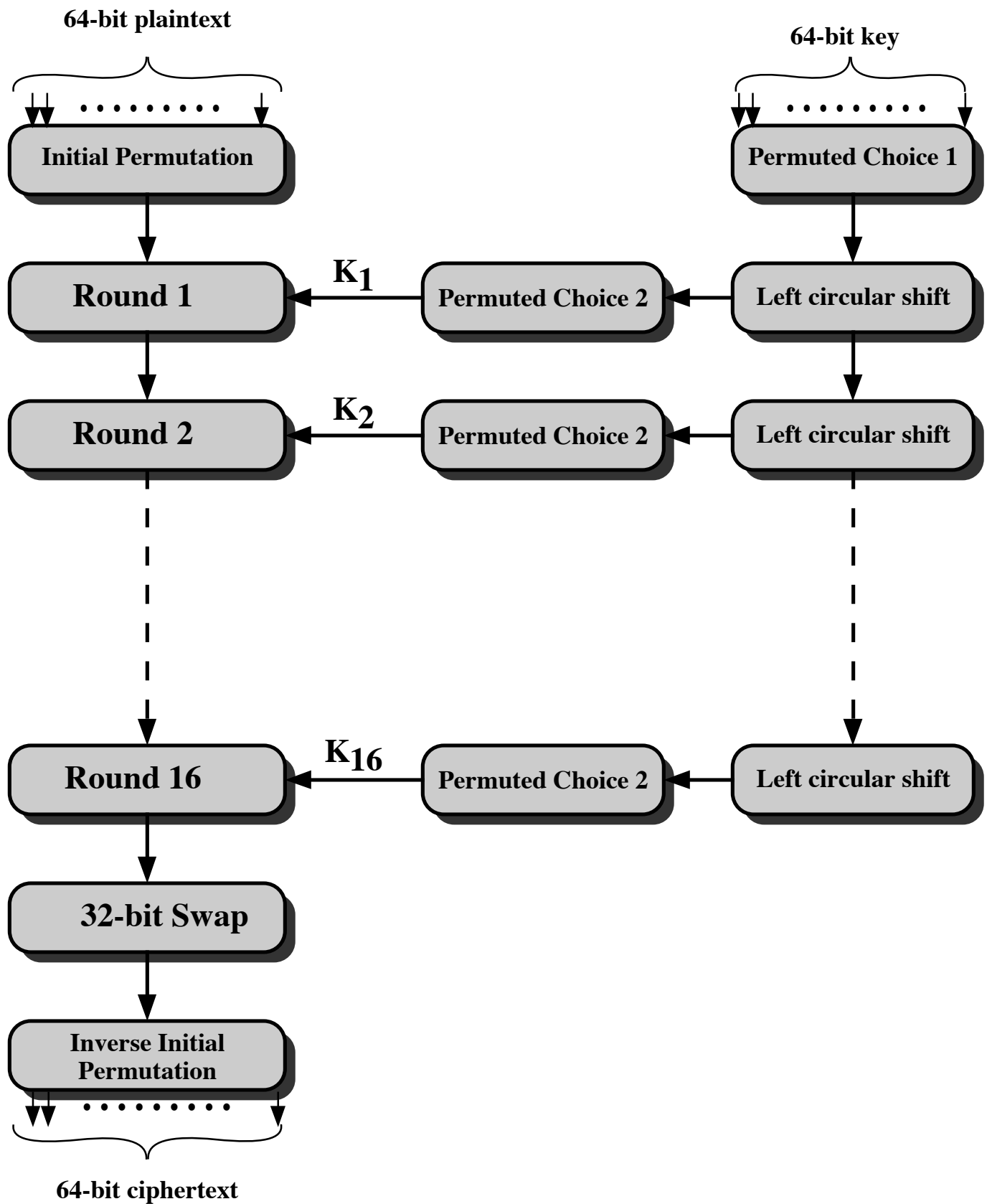
Figure 3.7 General Depiction of DES Encryption Algorithm
