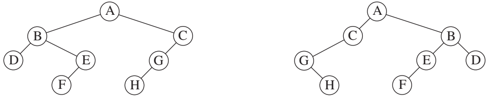
Figure 4.78 Two isomorphic trees
