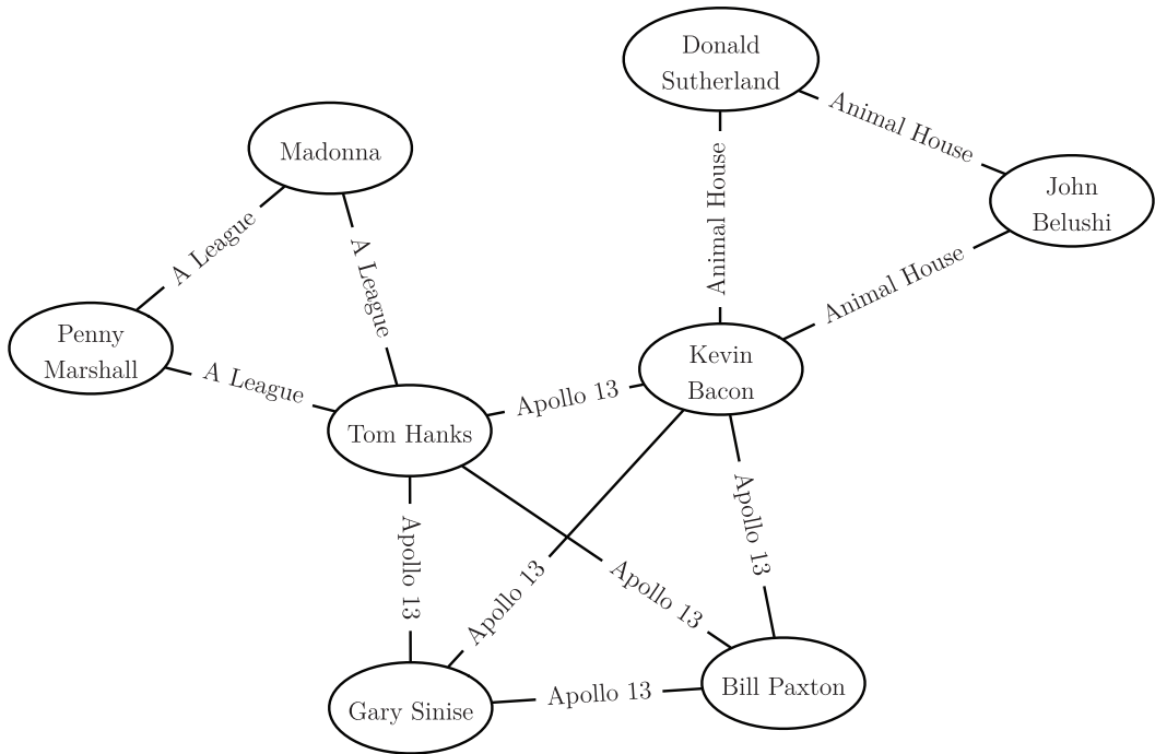
Figure 12.12 A simple actors network.
