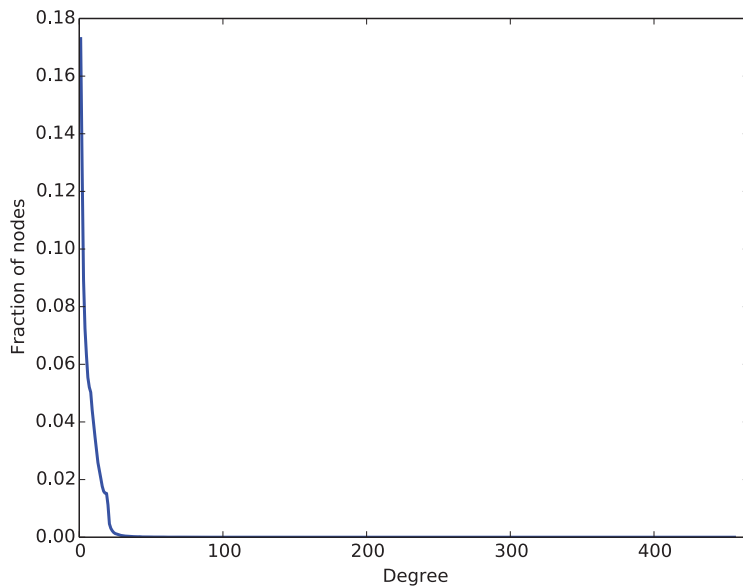
Figure 12.8. The degree distribution of 875,713 nodes in the web network.
