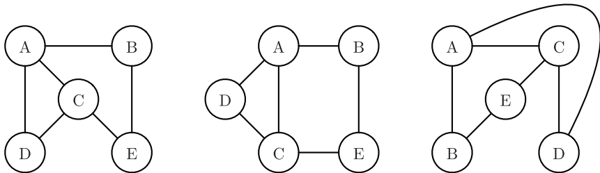
Figure 12.1 Three representations of the same graph.
