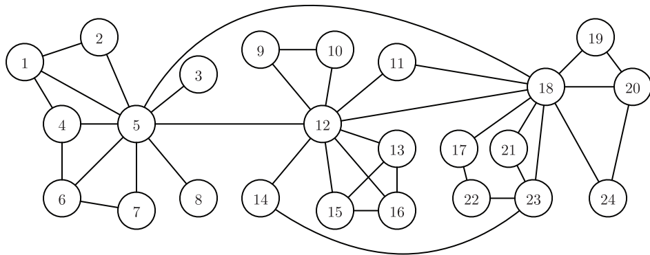
Figure 12.6 A small-world network.
