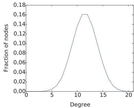
Figure 12.11. The degree distribution of random graphs with n = 24 and p = 1/2 .
