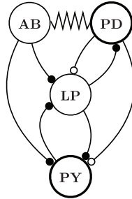
Figure 12.3 A model of the pyloric central pattern generator that controls stomach motion in lobsters.
