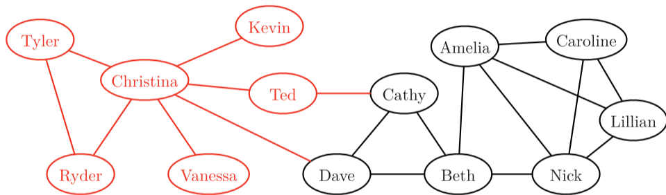
Figure 12.5 An expanded social network. The nodes and links in red are additions to the graph in Figure 12.2
