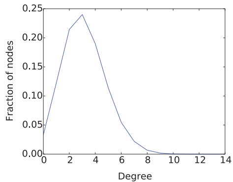
Figure 12.10 The degree distribution of random graphs with n = 24 and p = 38/276 .
