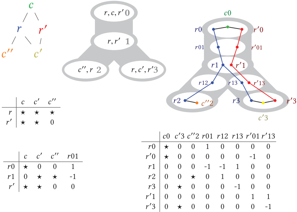
Fig. 2. On the left: a matrix M , its bipartite graph G_M , and the matrix after splitting the row r once (into r_0 and r_1 , creating the auxiliary column r_{01} ). In the middle: a tree decomposition of G_M with nodes 0, 1, 2, 3. On the right: the matrix after splitting according to this decomposition, and its graph in a tree-partition decomposition. The resulting graph is also a tree-split of G_M , with the constituent trees colored with the color of the corresponding vertex (since c, c', c'' appear in unique bags of the decompositions, their splittings are trivial, with one vertex and no edge, so no corresponding row appears).
