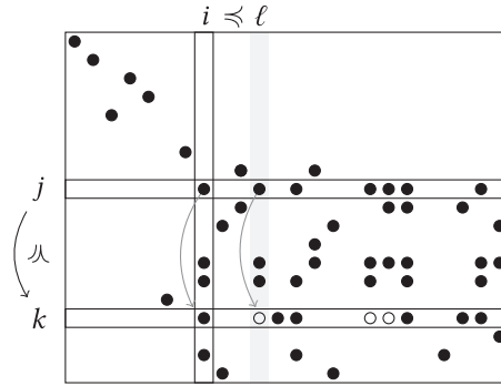
Fig. 1. The positions of non-zero entries (black circles) after a few steps of the algorithm. In the current step the entry in column i , row k will be eliminated using the earlier row j —entries that will become non-zero are marked as white circles.
