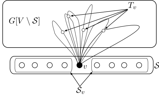
FIG. 5.2. The hitting set in Selective Flower Rule
