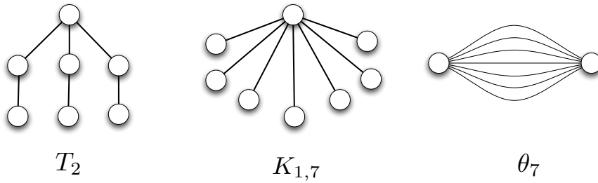
FIG. 1.1. Graphs T_2 , t -claw K_{1,t} with t = 7 , and \theta_c with c = 7
