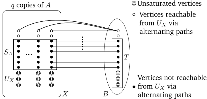
FIG. 5.1. The construction used in the proof of the q -Expansion Lemma
