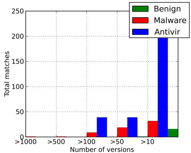
Fig. 6. Yield of different thresholds in the Mutating Payloads technique.
