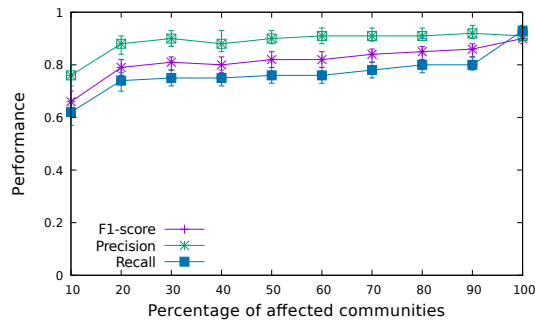
Figure 10: Effective in early detection of spam messages
