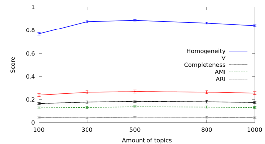
Figure 6: The metrics’ score slightly increase for 500 topics.
