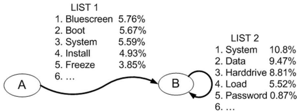
Figure 8: Expertise Awareness Example
