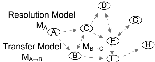
Figure 2: Unified Network Model
