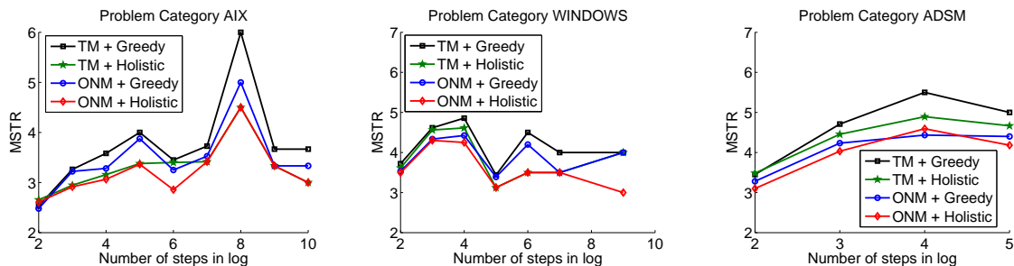
Figure 6: Routing Efficiency: Greedy Transfer vs. Holistic Routing
