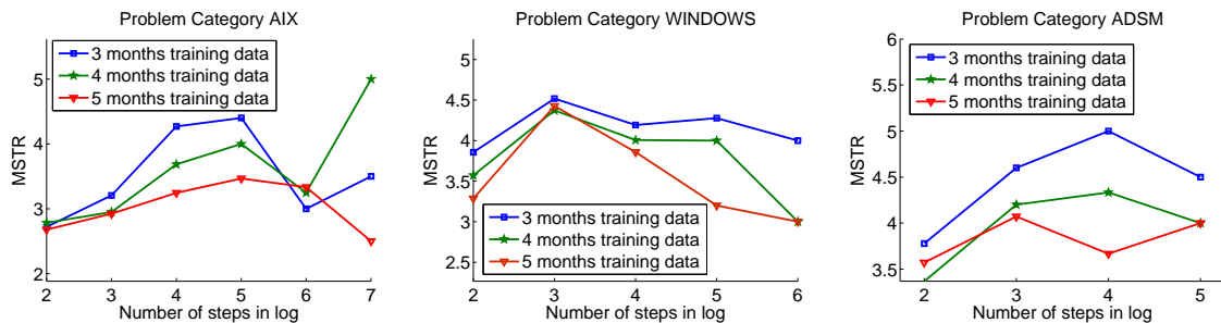
Figure 7: Robustness of ONM and Holistic Routing with Variable Training Data
