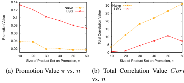
Figure 3: Product Selection Results on CH-SMarket Set
