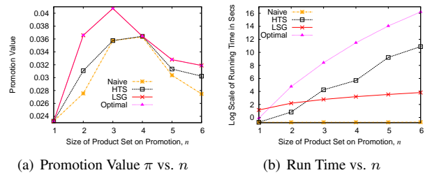
Figure 2: Product Selection Results on Synth Set
