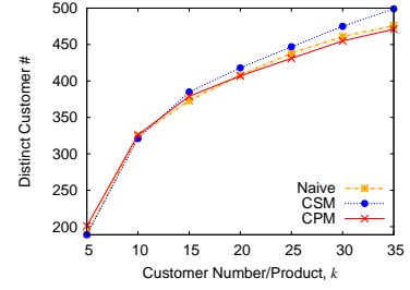
Figure 6: Distinct Customer No. vs. k on CH-Market Set
