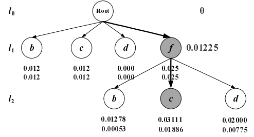
Figure 1: Applying HTS on Example in Table 2
