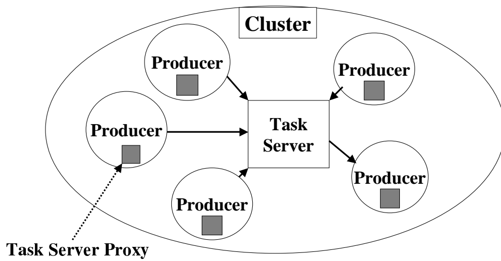
Figure 3: A Task server and its associated set of Producers.
