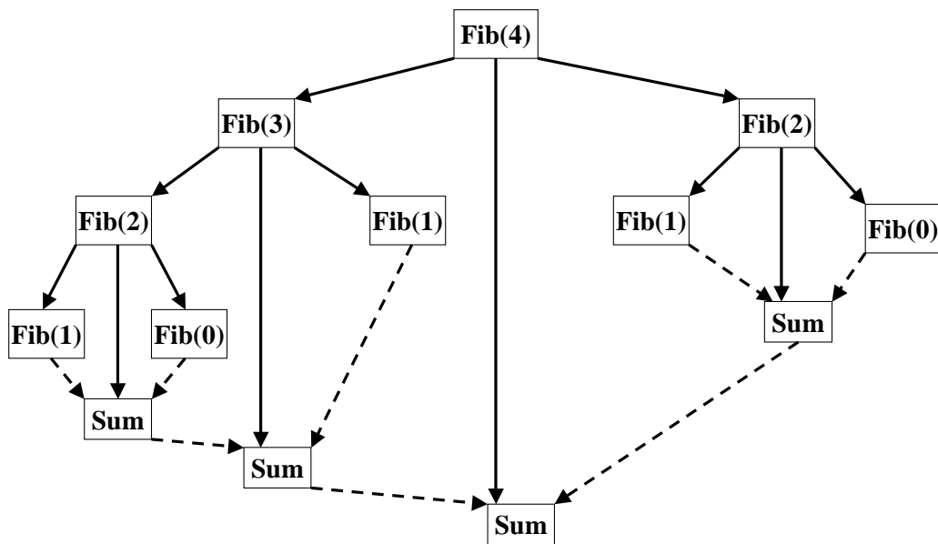
Figure 1: Task DAG for computing the 4th Fibonacci number.
