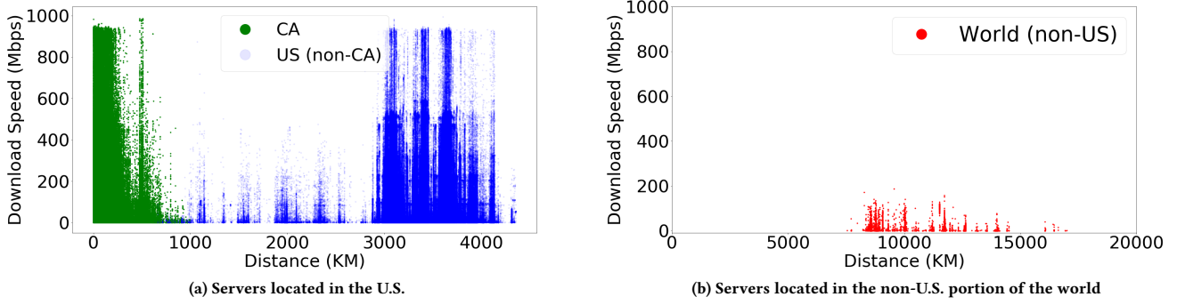
Figure 2: Download Speed of Measurements for Different Server Locations.
