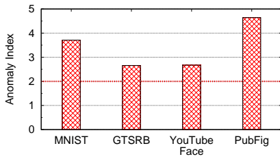
Fig. 11. Anomaly index of infected MNIST, GTSRB, YouTube Face, and PubFig model with noisy square trigger.
