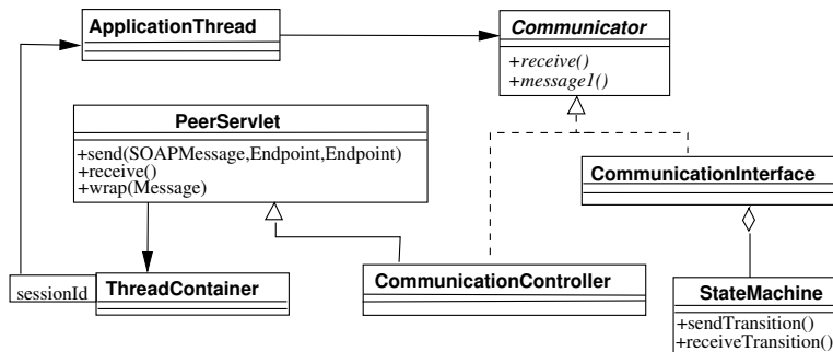
Fig. 4. Peer Controller Pattern Class Diagram
