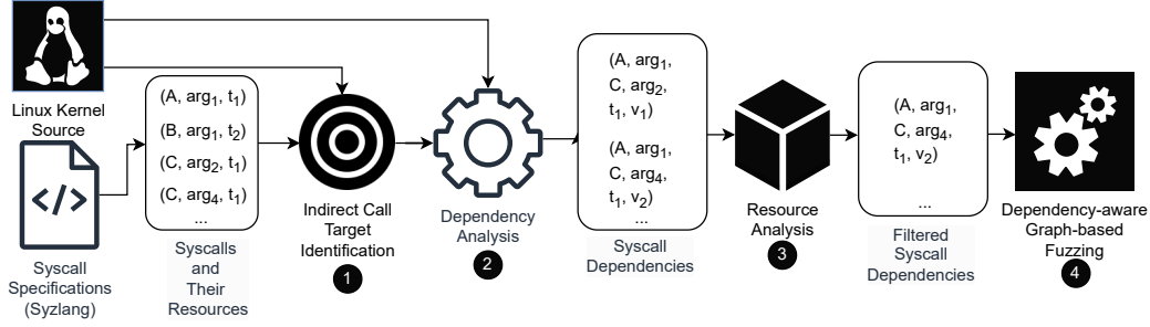
Fig. 3. The workflow of SYZGRAPHER.
