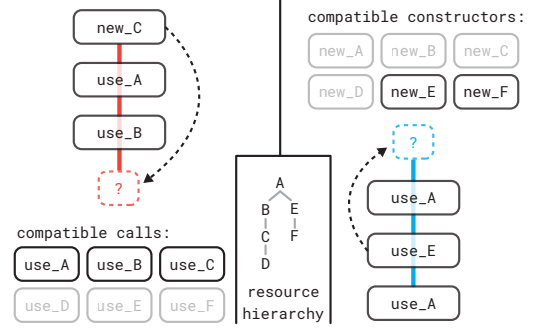
Fig. 6. Example graph extension in the forward direction (left) and reverse direction (right). The resource hierarchy tree is shown in the center. Dashed arrows show the existing syscall which enforces the constraint.
