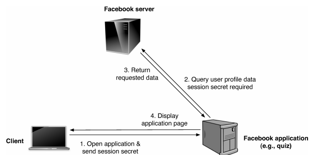
Figure 1: Data-flow in Facebook
