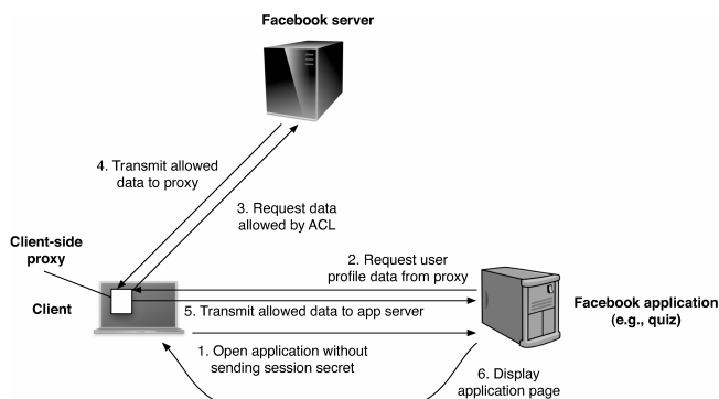
Figure 2: Modified data-flow with PoX
