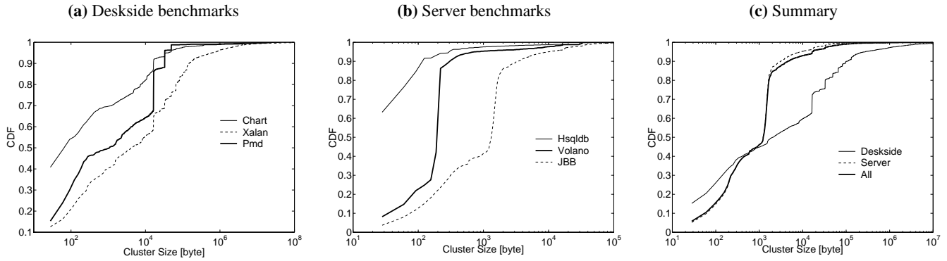
Figure 3. Distribution of cluster sizes for the desktside benchmarks (a), server benchmarks (b) and across the benchmarks (c). We report a CDF for each individual benchmark as well as summary CDFs for the desktside, server, and all benchmarks.
