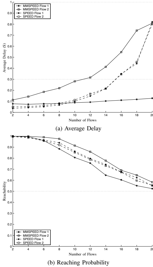
Fig. 4. Timeliness Differentiation.
