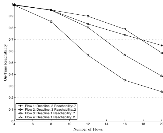
(a) MMSPEED
