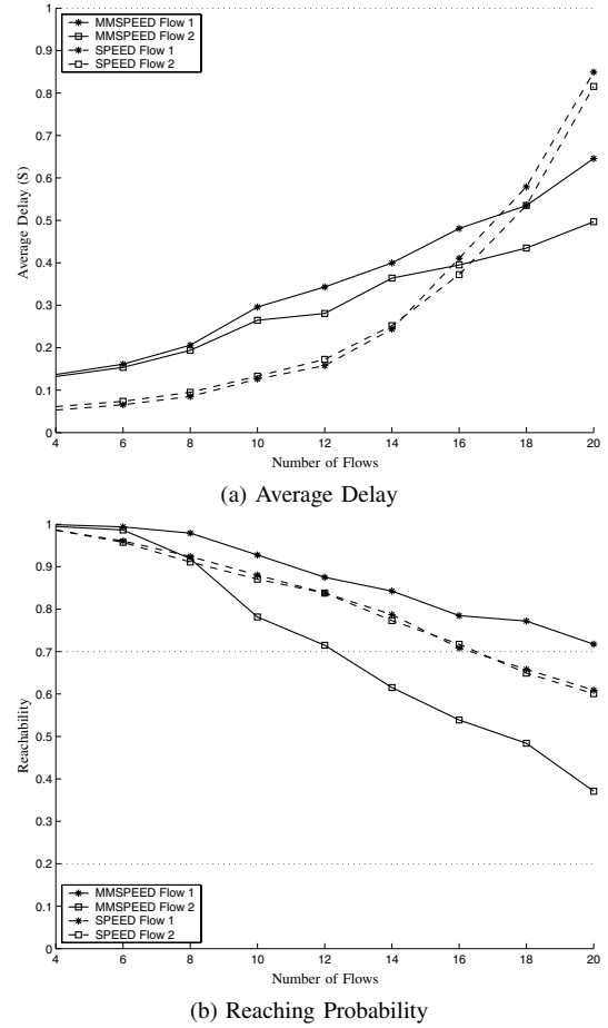
Fig. 5. Reliability Differentiation.
