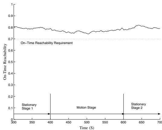
Fig. 9. Adaptability of MMSPEED.
