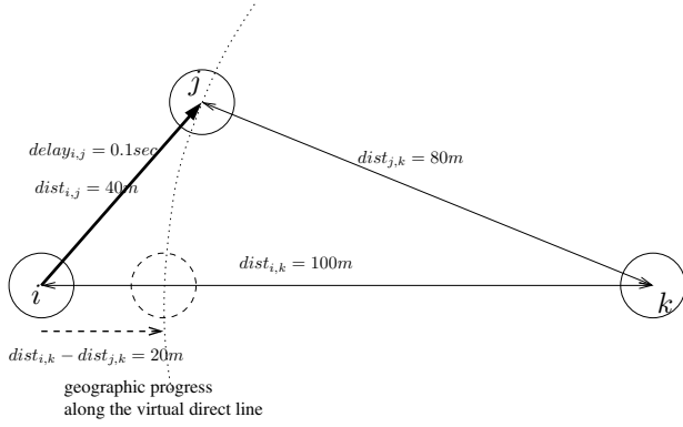
Fig. 1. Progress Speed from Node i to Node j toward Destination k .
