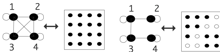
Figure A.3: A dense and a sparse matrix, both with their adjacency graph
