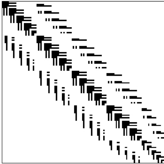
Figure 4.3: A matrix from an irregular problem
