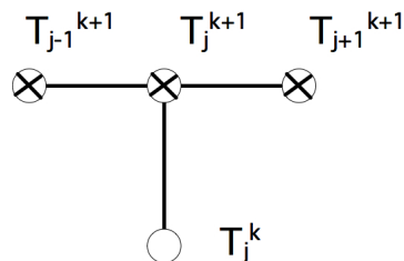
Figure 4.6: The difference stencil of the Euler backward method for the heat equation
