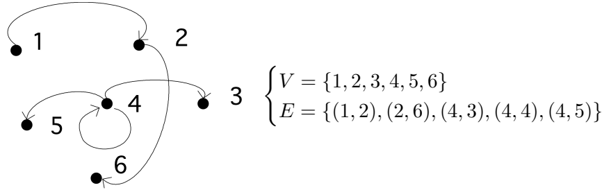
Figure A.1: A simple graph
