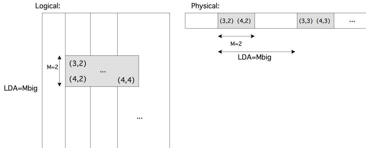
Figure B.3: A subblock out of a larger matrix, using LDA
