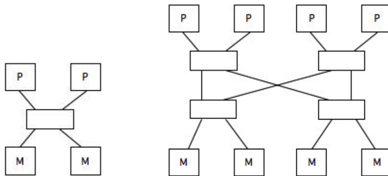
Figure 2.19: A butterfly exchange network for two and four processors/memories
