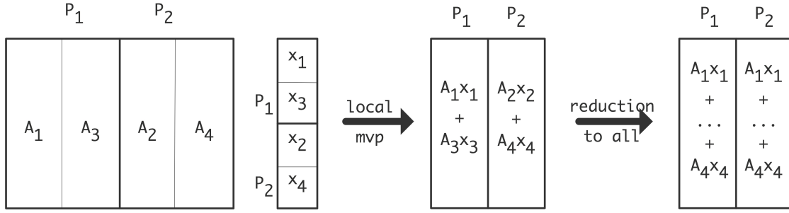
Figure 6.5: Matrix-vector multiplication with a cyclicly distributed matrix
