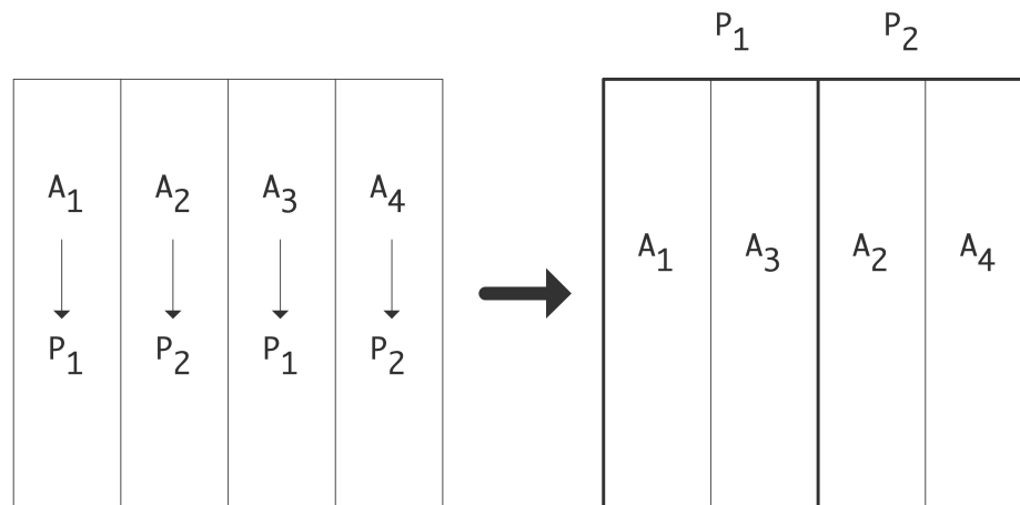
Figure 6.4: One-dimensional cyclic distribution: assignment of four matrix columns to two processors, and the resulting mapping of storage to matrix columns
