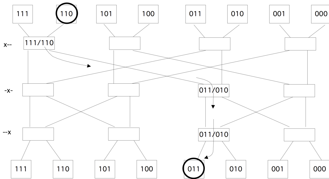
Figure 2.21: Routing through a three-stage butterfly exchange network
