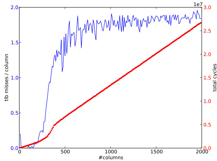
Figure 1.11: Number of TLB misses per column as function of the number of columns; columnwise traversal of the array.
