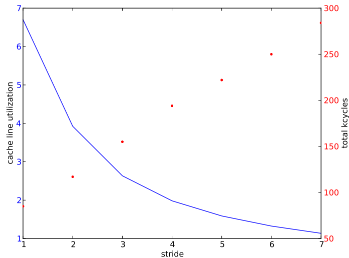
Figure 1.10: Run time in kcycles and L1 reuse as a function of stride
