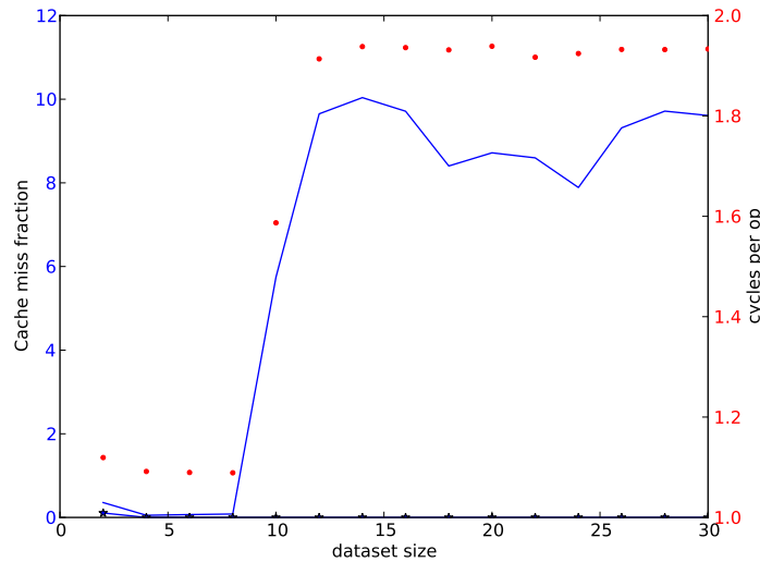
Figure 1.9: Average cycle count per operation as function of the dataset size
