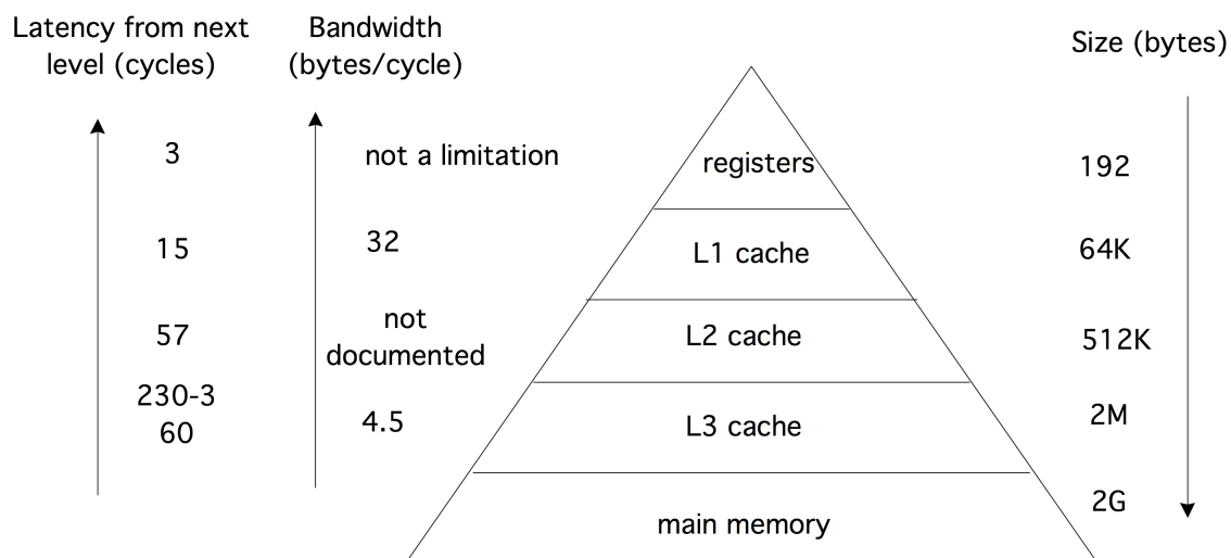
Figure 1.3: Memory hierarchy of an AMD Xeon, characterized by speed and size.
