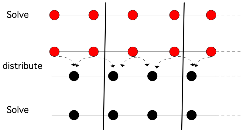
Figure 6.15: Parallel red-black solution on a 1d domain
