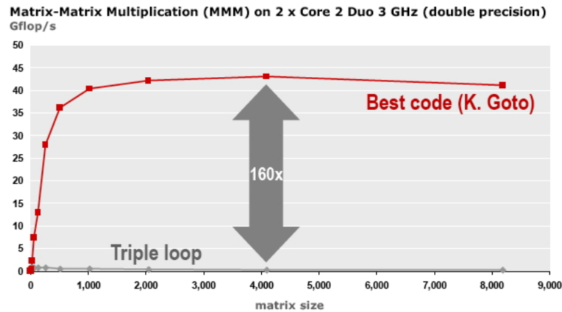
Figure 1.16: Performance of naive and optimized implementations of the matrix-matrix product
