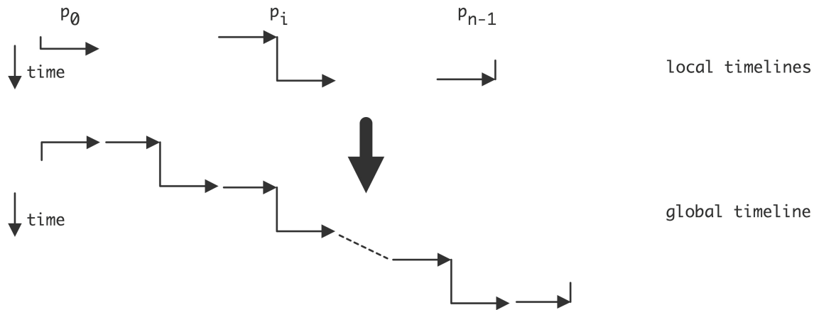
Figure 2.9: Local and resulting global view of an algorithm for sending data to the right
