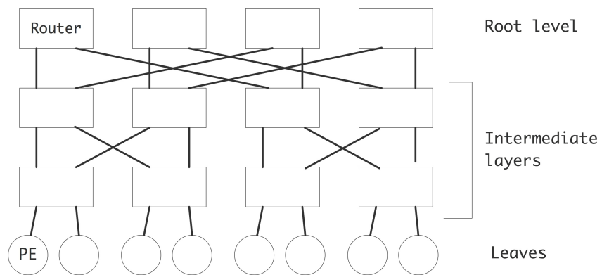
Figure 2.23: A fat-tree built from simple switching elements
