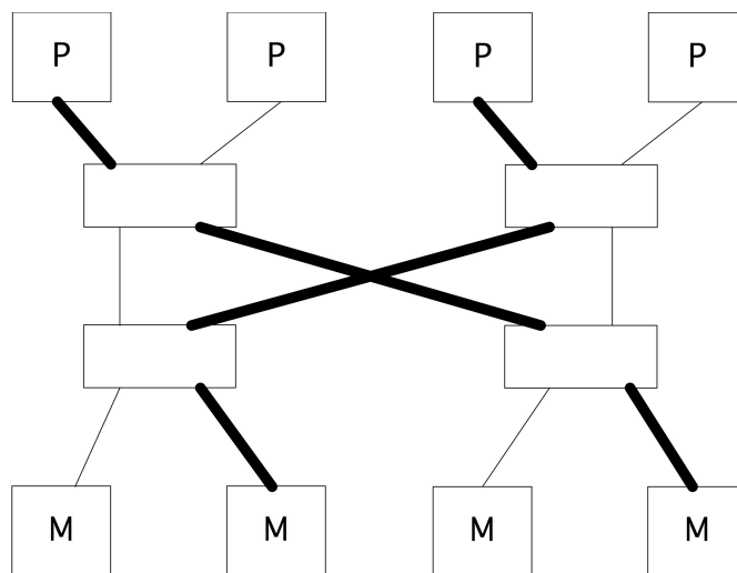
Figure 2.20: Two independent routes through a butterfly exchange network
