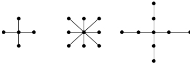
Figure 4.4: The structure of some difference stencils in two dimensions
