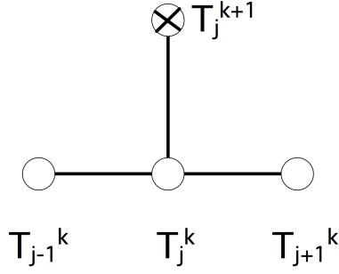
Figure 4.5: The difference stencil of the Euler forward method for the heat equation
