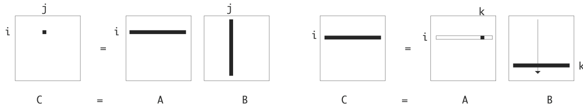
Figure 1.8: Two loop orderings for the C \leftarrow A \cdot B matrix-matrix product
