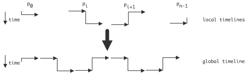
Figure 2.11: Local and resulting global view of an algorithm for sending data to the right
