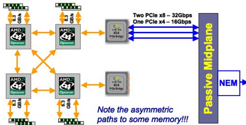
Figure 2.4: Non-uniform memory access in a four-socket motherboard
