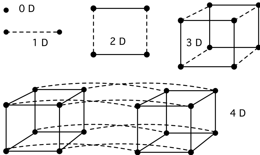
Figure 2.15: Hypercubes
