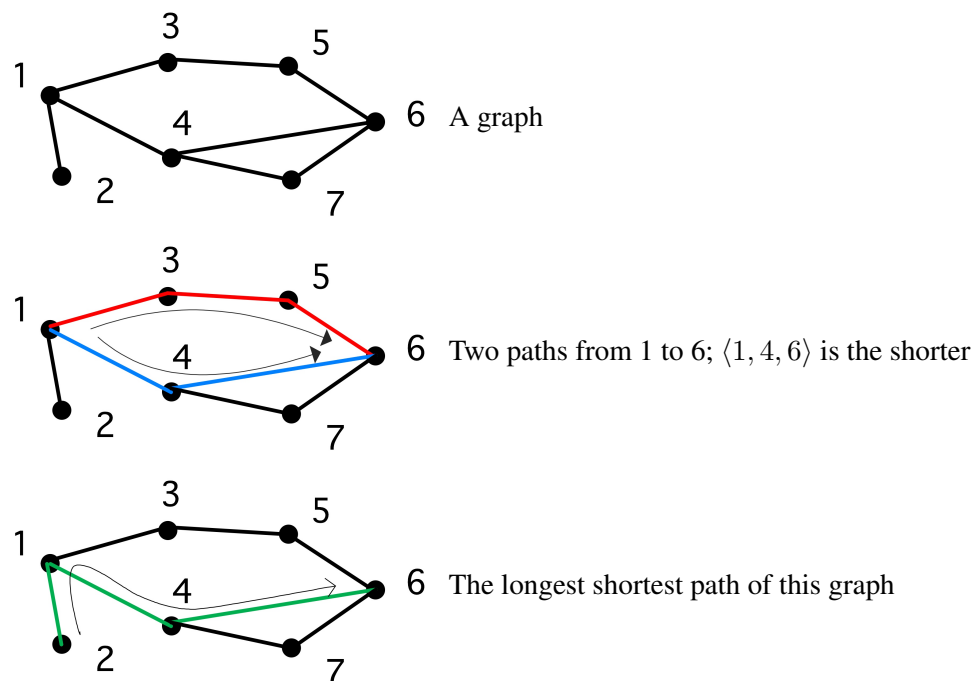
Figure A.2: Shortest paths
