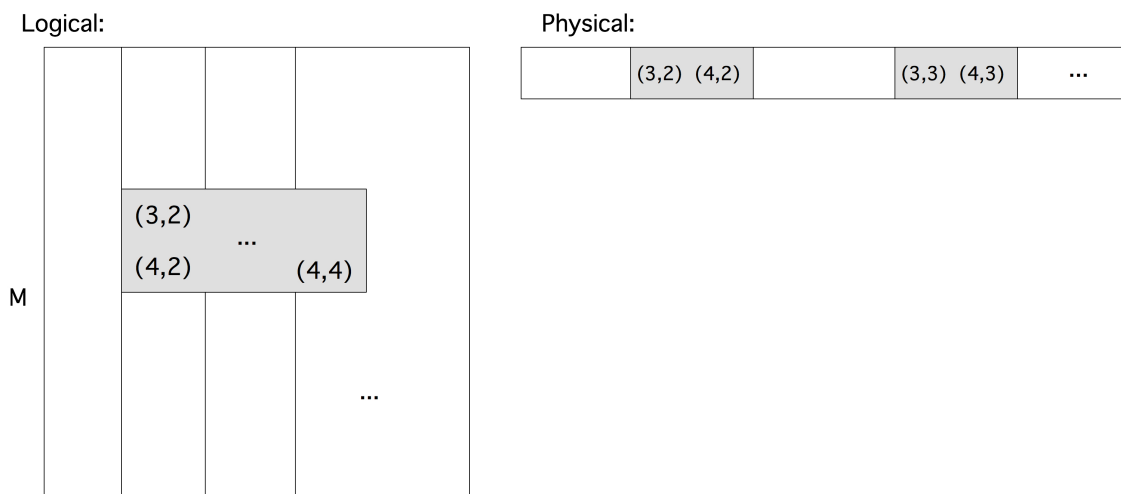
Figure B.2: A subblock out of a larger matrix
