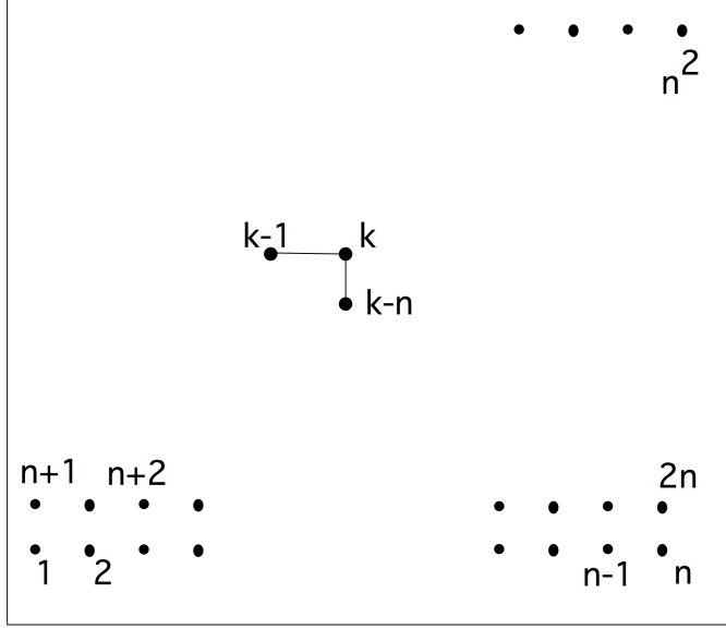
Figure 6.17: The difference stencil of the L factor of the matrix of a two-dimensional BVP
