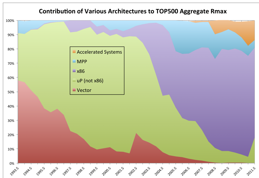
Figure 2.29: Evolution of the architecture types on the top500 list
