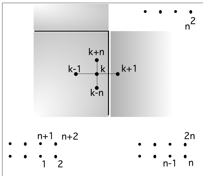
Figure 6.6: A difference stencil applied to a two-dimensional square domain, distributed over processors. A cross-processor connection is indicated.
