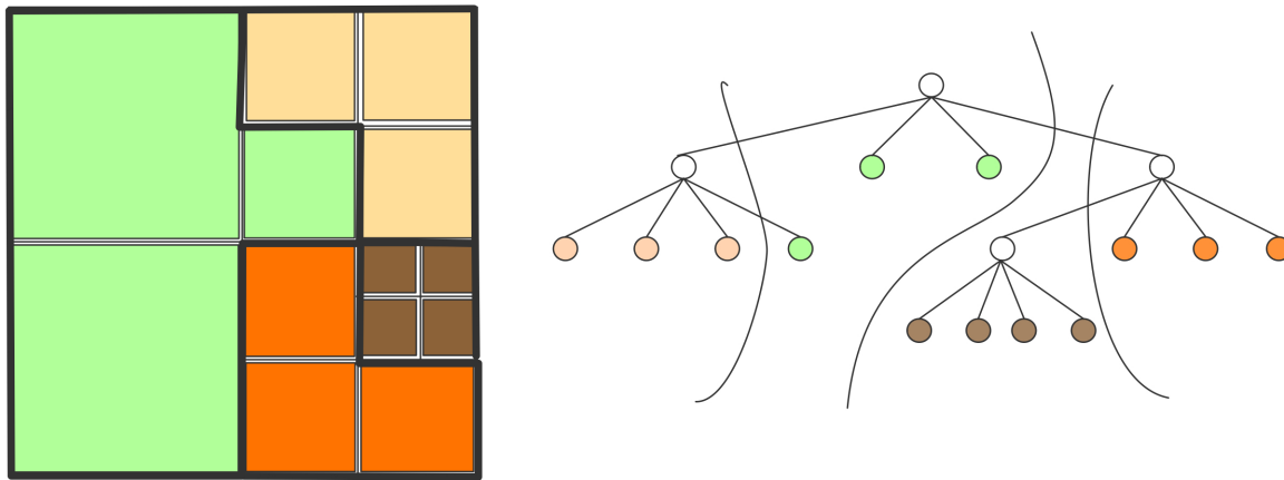
Figure 2.26: Load distribution of an adaptively refined domain
