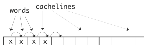
Figure 1.4: Accessing 4 elements at stride 1
