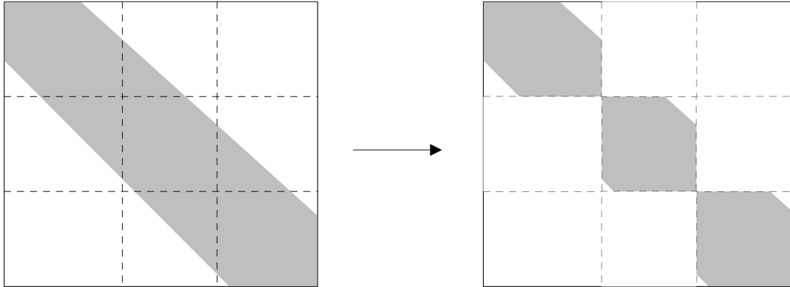
Figure 6.9: Sparsity pattern corresponding to a block Jacobi preconditioner
