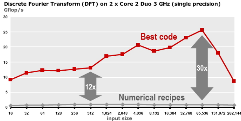
Figure 1.15: Performance of naive and optimized implementations of the Discrete Fourier Transform
