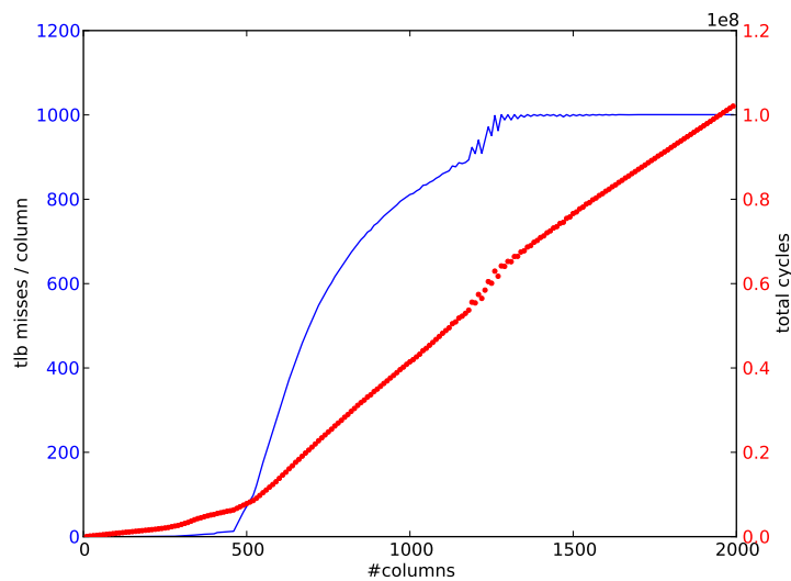
Figure 1.12: Number of TLB misses per column as function of the number of columns; rowwise traversal of the array.
