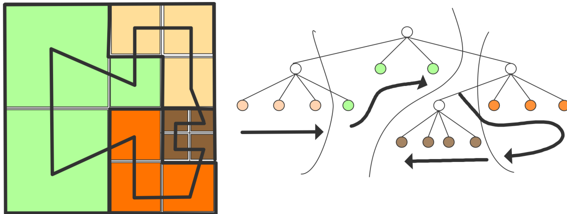
Figure 2.27: A space filling curve for the load balanced tree
