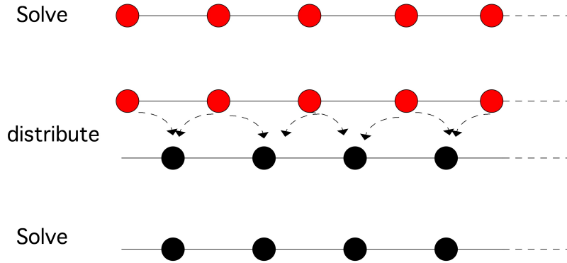
Figure 6.14: Red-black solution on a 1d domain
