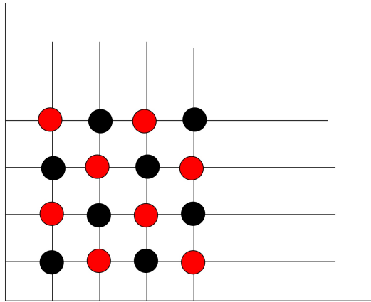
Figure 6.16: Red-black ordering of the variables of a two-dimensional domain
