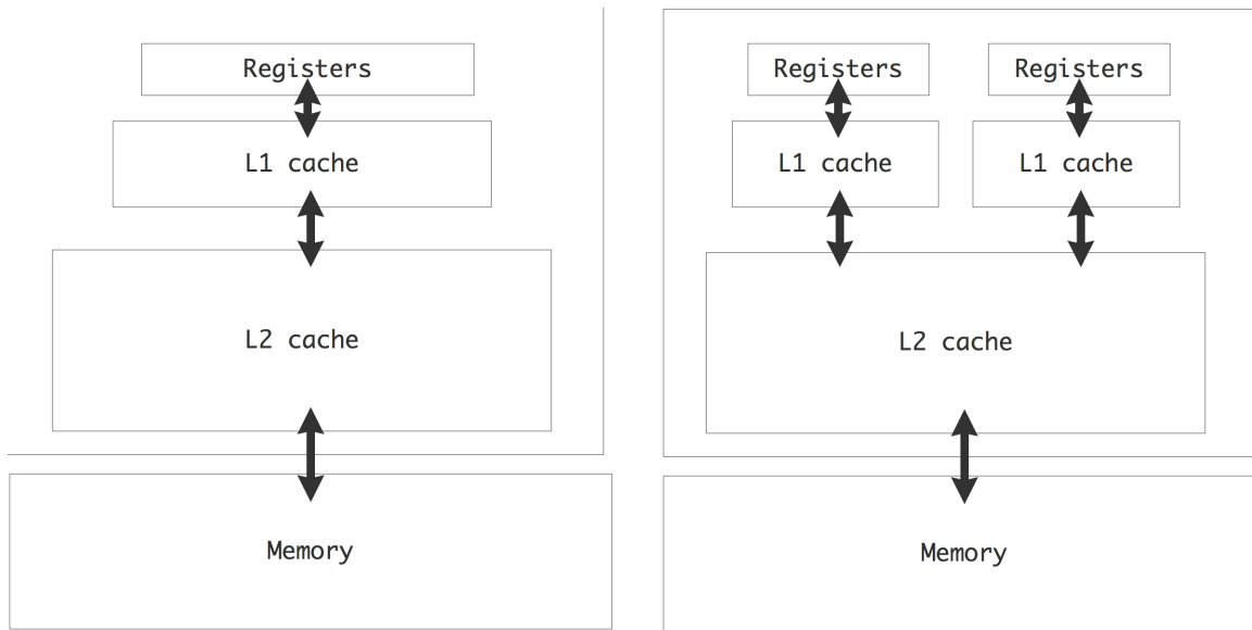
Figure 1.2: Cache hierarchy in a single-core and dual-core chip
