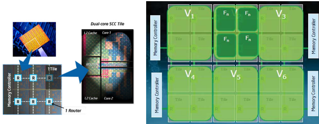
Figure 1.7: Structure of the Intel Single-chip Cloud Computer chip
