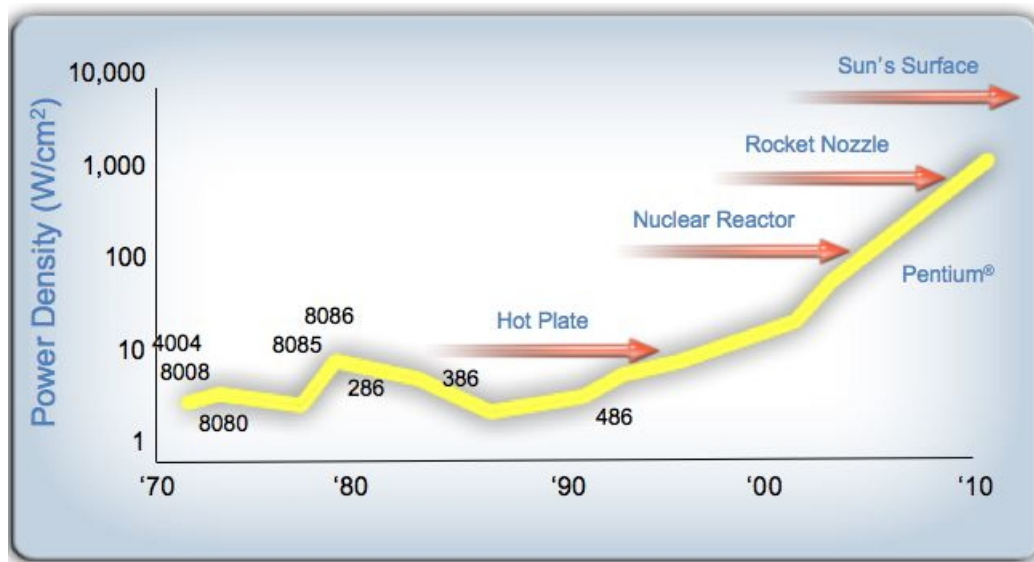
Figure 1.17: Projected heat dissipation of a CPU if trends had continued – this graph courtesy Pat Helsingier illustration of the heat that a chip would give off, if single-processor trends had continued.
