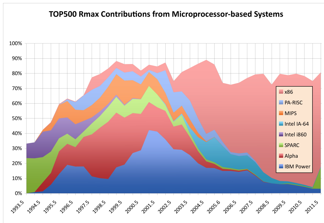
Figure 2.30: Evolution of the architecture types on the top500 list
