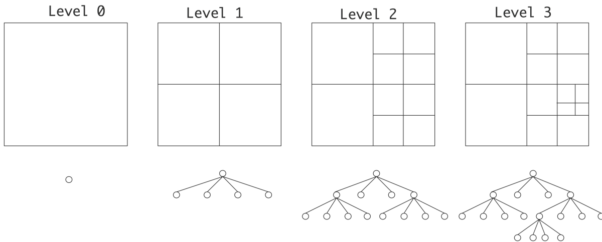
Figure 2.25: Adaptive refinement of a domain in subsequent levels
