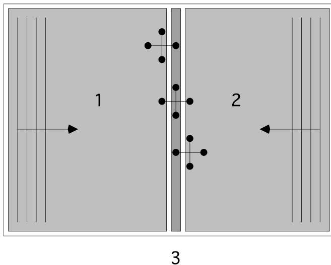
Figure 6.10: Domain dissection into two unconnected subdomains and a separator
