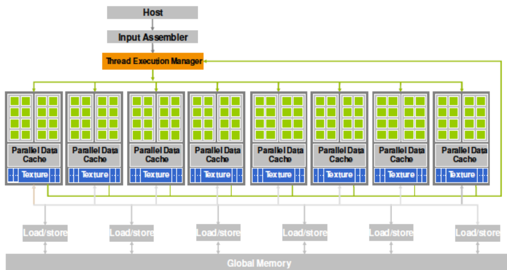
Figure 2.24: Diagram of a GPU
