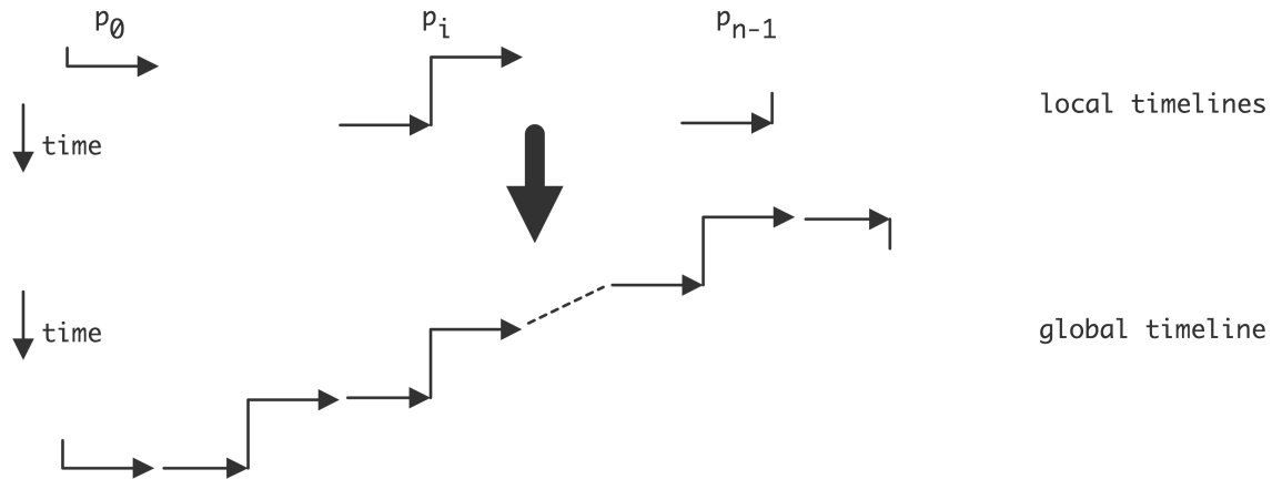
Figure 2.10: Local and resulting global view of an algorithm for sending data to the right
