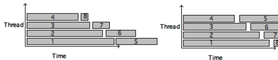
Figure 2.8: Static or round-robin (left) vs dynamic (right) thread scheduling; the task numbers are indicated.
