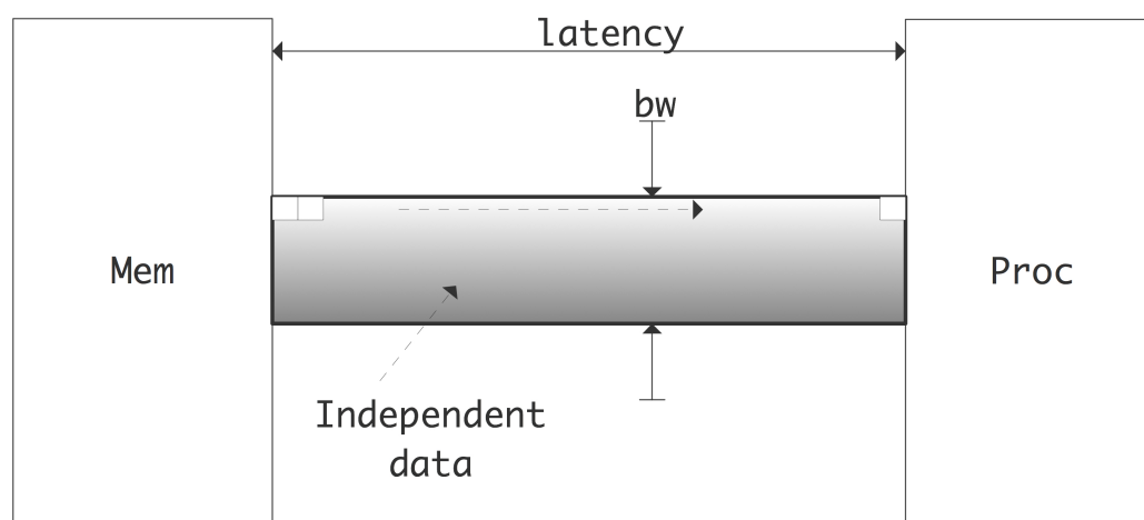
Figure 1.6: Illustration of Little's Law that states how much independent data needs to be in flight
