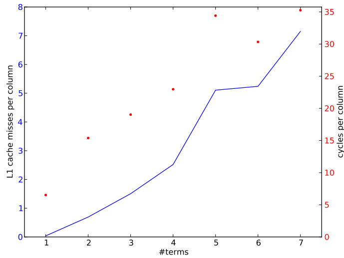
Figure 1.13: The number of L1 cache misses and the number of cycles for each j column accumulation, vector length 4096
