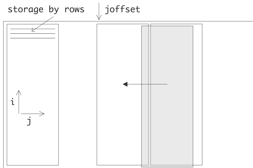
Figure 2.12: Data shift that requires communication
