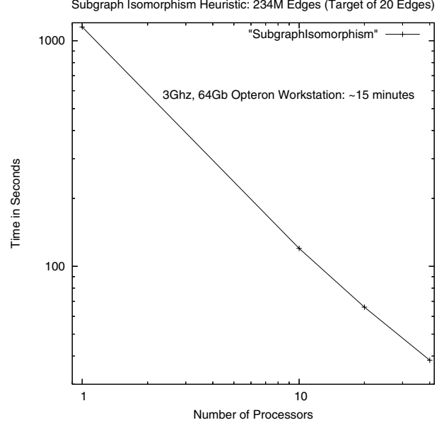
Figure 17: Subgraph isomorphism kernel performance
