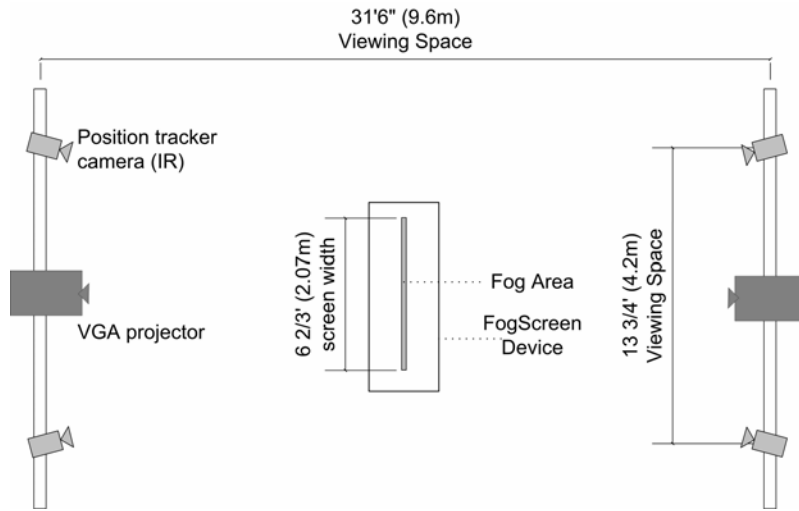
Figure 3: The dual-sided prototype system setup.
