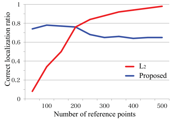
Figure 2: Localization results for the proposed method and L_2 -norm matching over all images.
