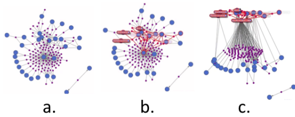
Figure 6. Example of EvoCut algorithm. Evocut is run on the blue node in the center of fig. a. The algorithm selects the highlighted cluster in b. which is then moved via the interpolation method shown in c.
