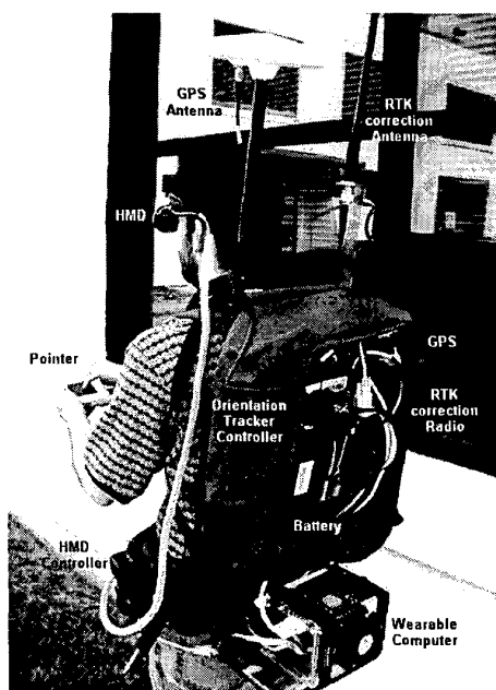
Figure 1. Prototype mobile AR system.
