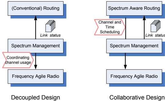
Fig. 1. System Design.
