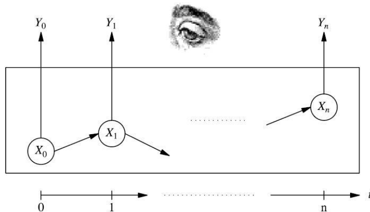
Hidden Markov Model
