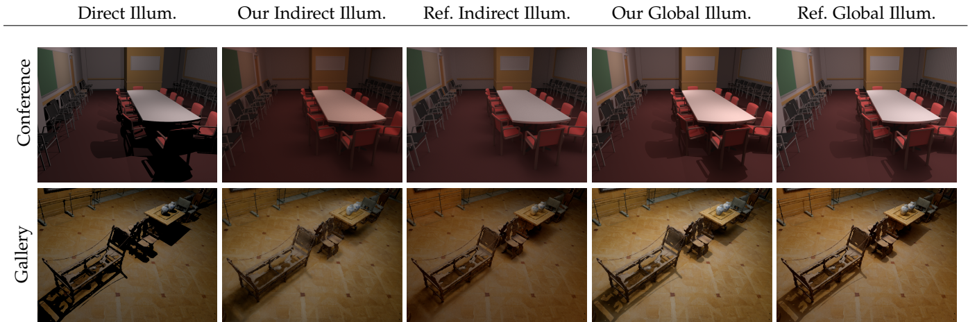
Fig. 8. Comparison of indirect illumination results between our method and the reference global illumination generated by path tracing. For each scene, from left to right, we provide the input direct illumination, our indirect illumination, reference indirect illumination, our global illumination, and reference global illumination.
