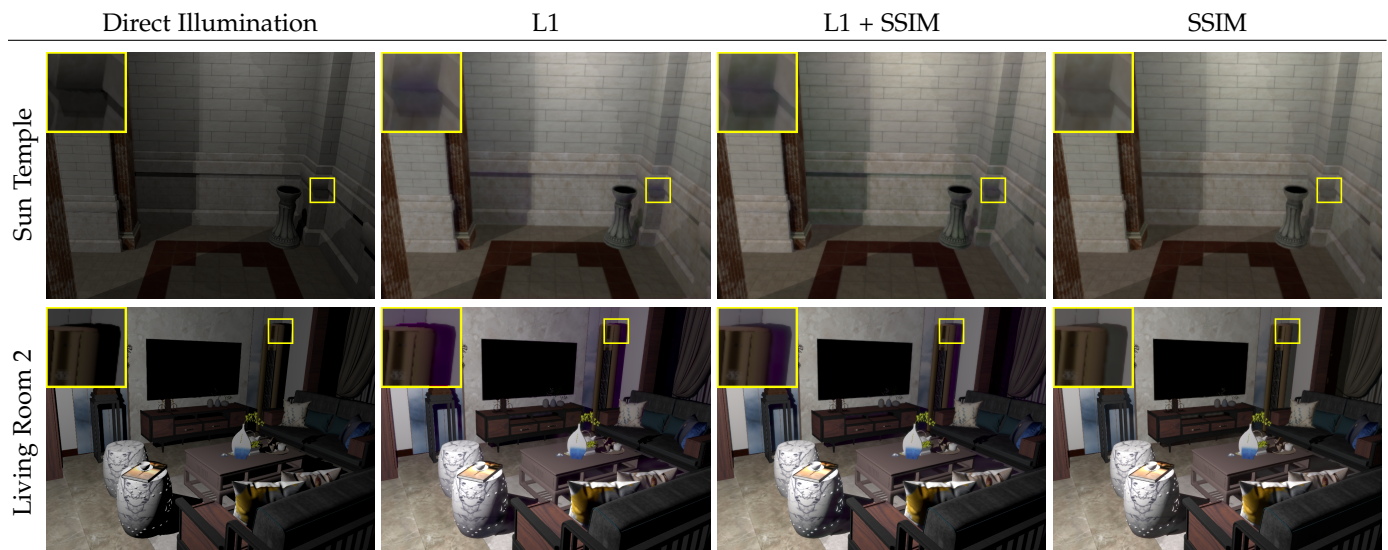
Fig. 11. Comparisons of different metrics in computing the content loss term (Equation 4). ‘Using L1 only’ or ‘using L1+SSIM’ are easy to introduce color-shifting artifacts in dark areas. ‘Using SSIM only’ generates results with the best visual quality.
