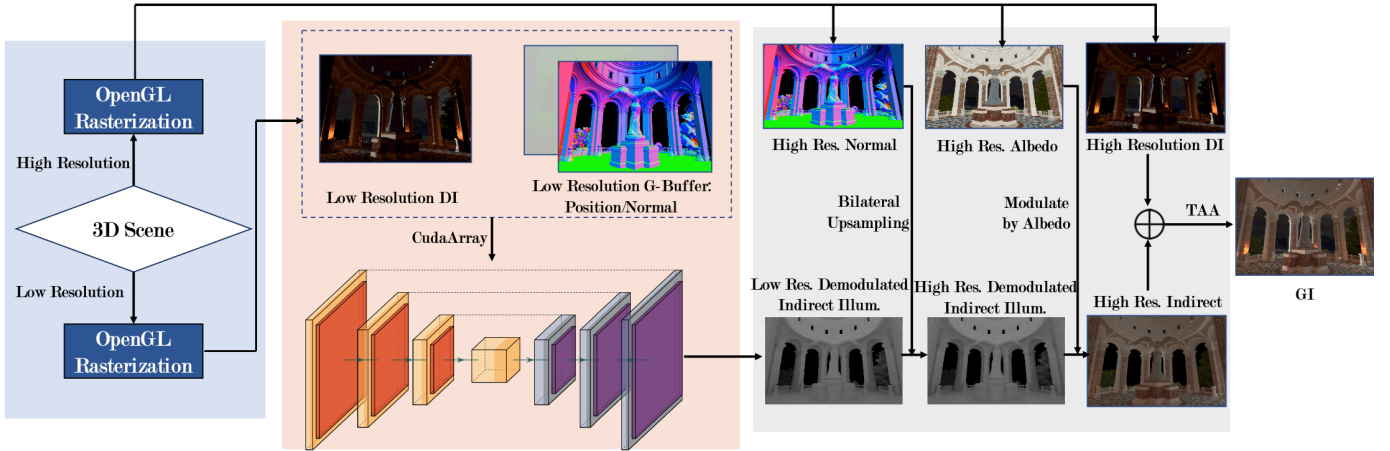
Fig. 6. Our rendering pipeline. We use OpenGL rasterization to generate both high-resolution (i.e., 1024 \times 768 ) and low-resolution (i.e., 512 \times 384 ) direct illumination with associated G-buffers. The low-resolution direct illumination and associated G-buffers are fed into our neural network to produce low-resolution demodulated indirect illumination. High-resolution normal/albedo maps are used to generate high-resolution indirect illumination through joint bilateral upsampling and albedo modulation. We then add the upsampled indirect illumination with the high-resolution direct illumination, and further apply Temporal Anti-Aliasing (TAA) to obtain the final high-resolution global illumination results.
