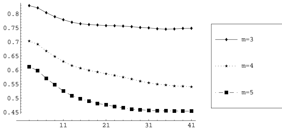
Figure 2. The probability that the Condorcet winner is also a Plurality winner in the IANC model. The raw data has been smoothed out by a 5-term moving-average filter. The horizontal axis is the number of voters n , through odd integers from 3 to 41. The number of samples used is k = 1000 per m/n pair.
