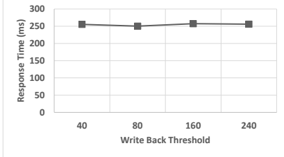
(e) Effect of write-back threshold on response time
