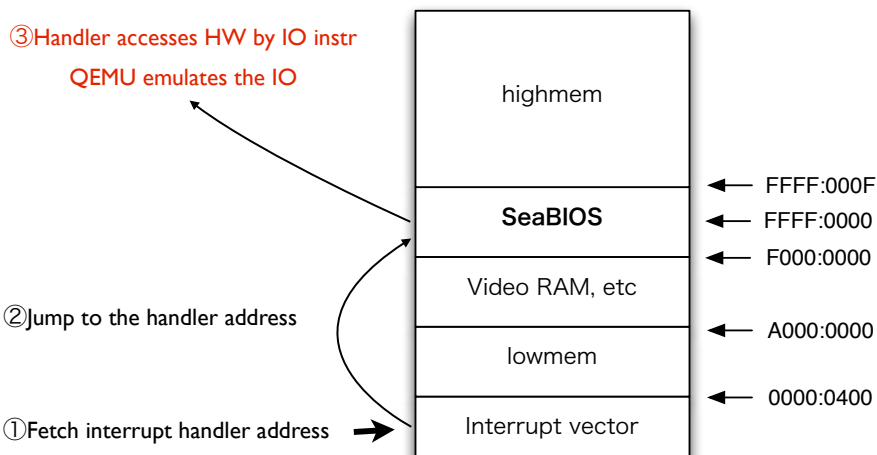
Figure 11. BIOS interrupt call mechanism on KVM
