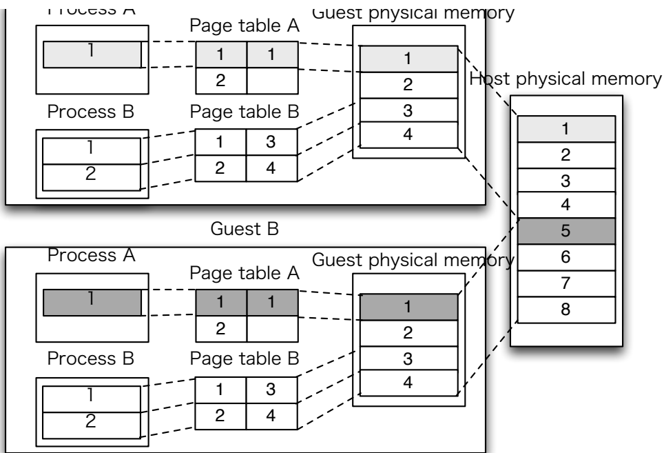
Figure 5. Problem of memory virtualization
