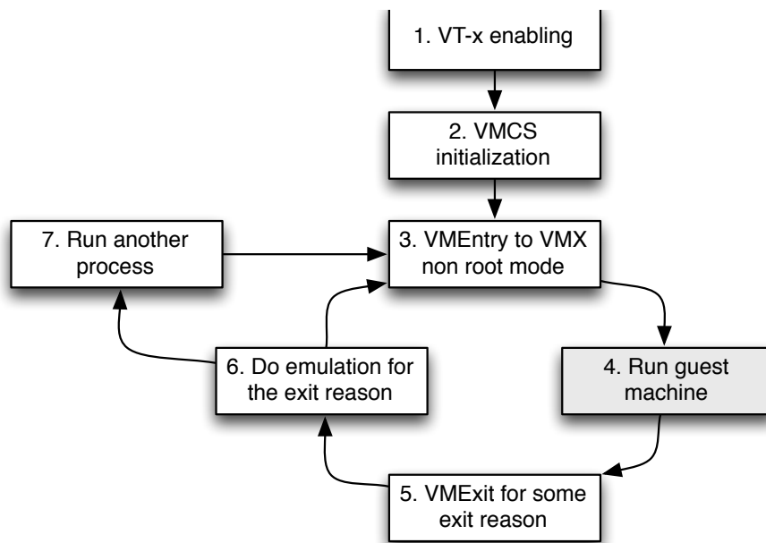
Figure 4. VT-x enabled hypervisor lifecycle
