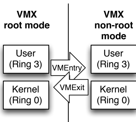
Figure 2. VMEntry and VMExit
