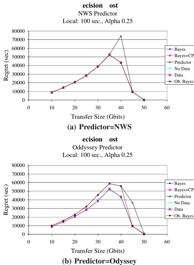
Fig. 6. Predictor performance (regret) for different task sizes and decision strategies for the 1Gb/s trace for predictors NWS (a) and Ody (b).
