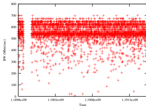
Fig. 5. Network bandwidth observations for 1Gb/s trace for first 5000 observations.
