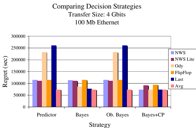
Fig. 4. Predictor performance (regret) for all prediction-based strategies for the critical bandwidth of 53Mb/s using the 100Mb/s network.
