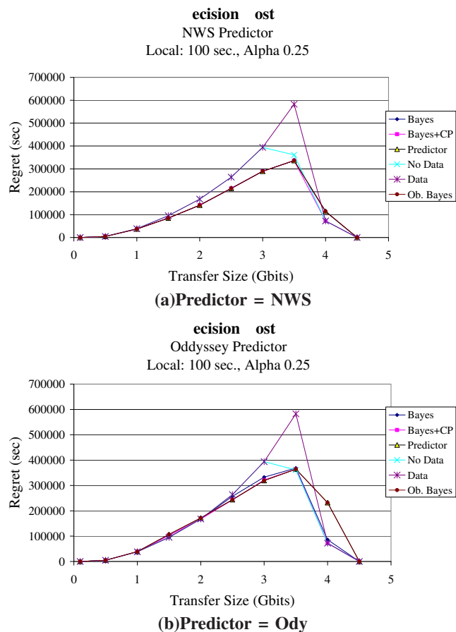
Fig. 3. Predictor performance (regret) for different task sizes and decision strategies for the 100Mb/s trace for predictors NWS (a) and Ody (b).
