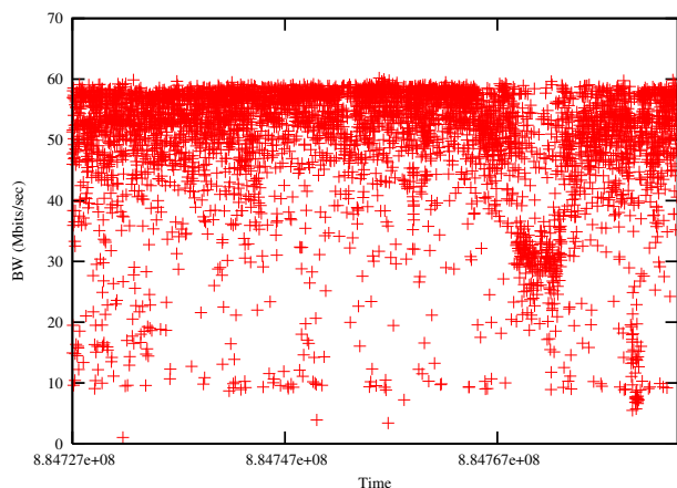
Fig. 2. Network bandwidth observations for 100Mb/s trace for first 5000 observations.
