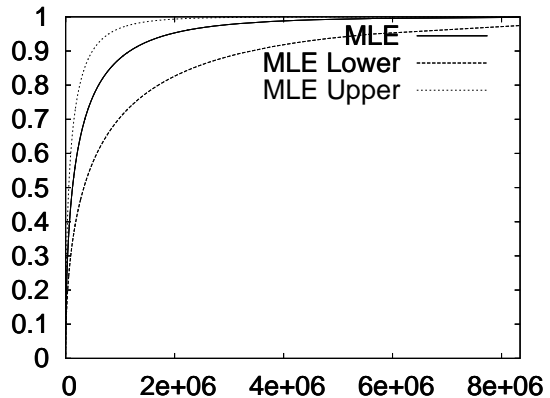
Figure 2: 90% Confidence Interval Graphs for Weibull shown in Figure 1 ( \alpha = 0.536852 and \beta = 249105 ).
