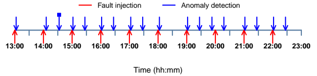
Figure 3: Anomaly detection in guestbook application during a period of 10 hours. Red arrows indicate fault injection at the datastore service. Blue arrows indicate all anomalies detected by Roots.
