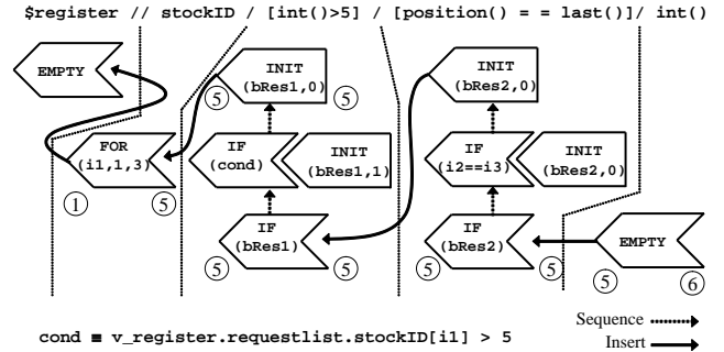
Figure 6: Code Sample
