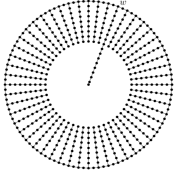
Figure 8: Lower bound graph
