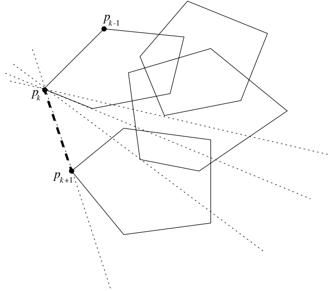
Figure 1: Wrapping a set of \lceil n/m \rceil convex polygons of size m .
