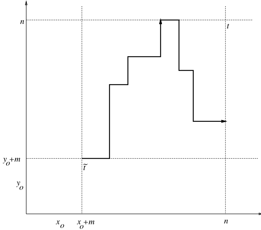
FIG. 3. The algorithm for the room problem. Here \tilde{t} = t' .
