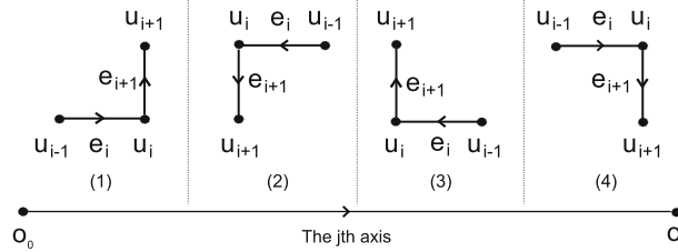
Fig. 5 Demonstration of 4 situations in Lemma 13
