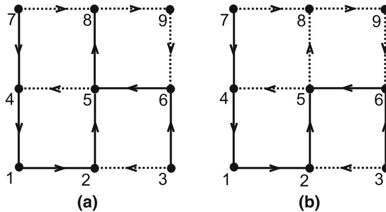
Fig. 1 Two nearly identical 2-colored lattice graphs, one observable (on left), the other non-observable (on right). The two colors are shown as solid (S) and dashed (D). Only the color of edge (5, 8) differs in the two graphs. In b, the color sequence (SSSD)* can lead to either node 4 or 8, making it non-observable. In a, any walk of dimension 4 is observable
