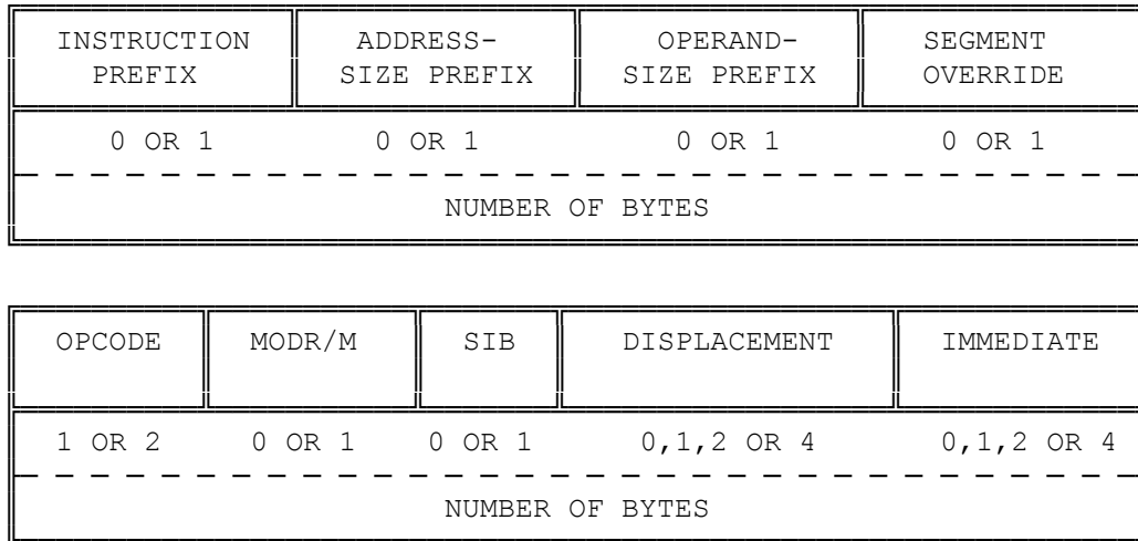
Figure 17-1. 80386 Instruction Format
