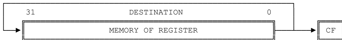
Figure 3-13. ROR
