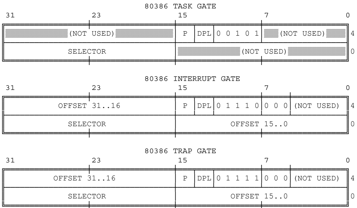
Figure 9-3. 80386 IDT Gate Descriptors
