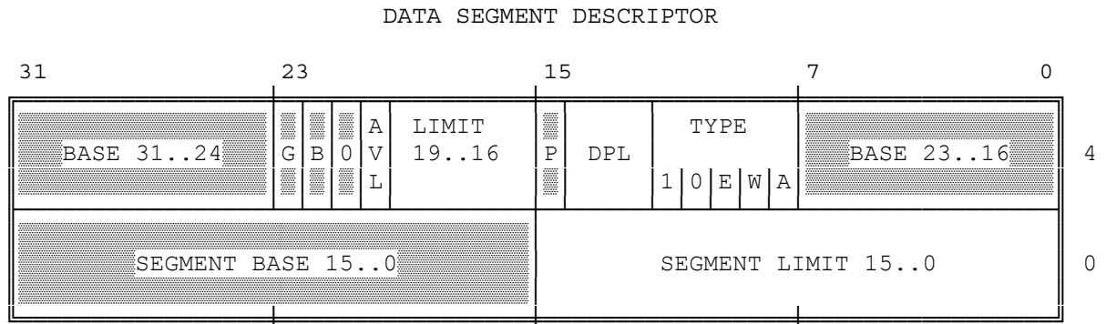
Figure 6-1. Protection Fields of Segment Descriptors
