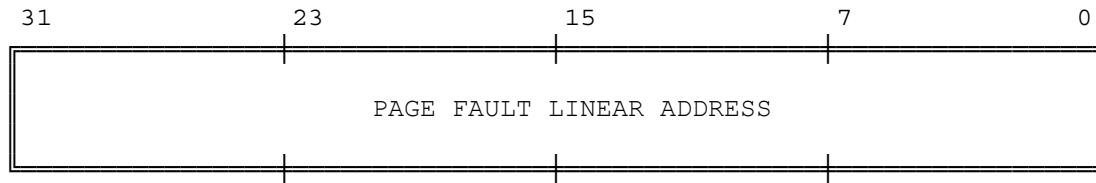
Figure 9-9. CR2 Format
