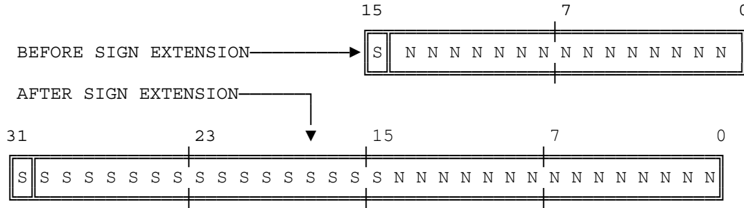
Figure 3-5. Sign Extension
