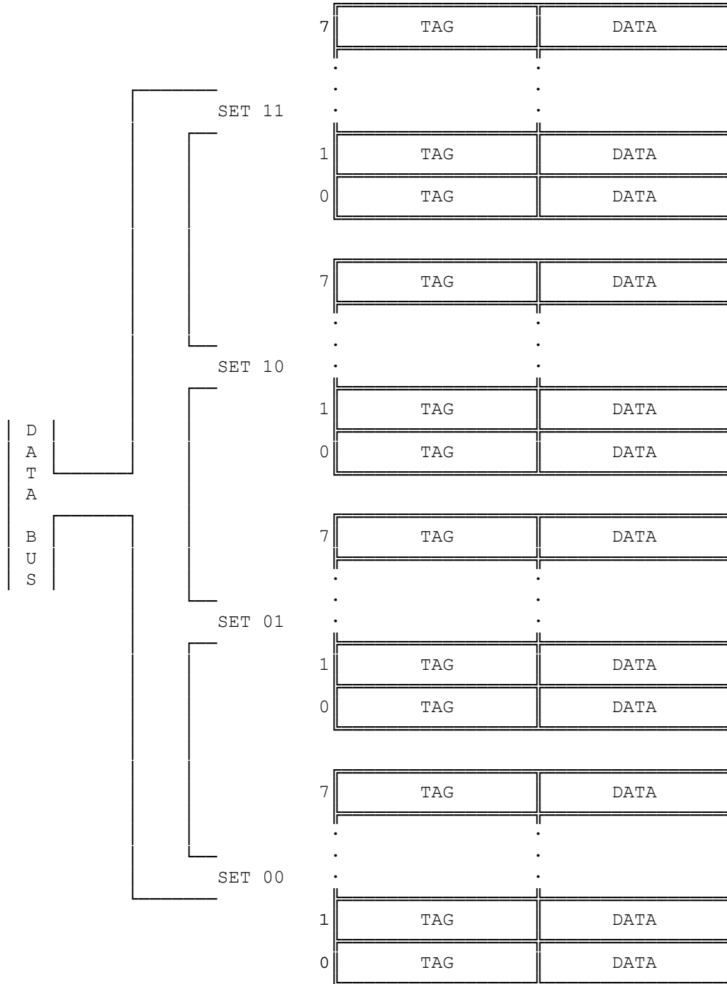
Figure 10-3. TLB Structure
