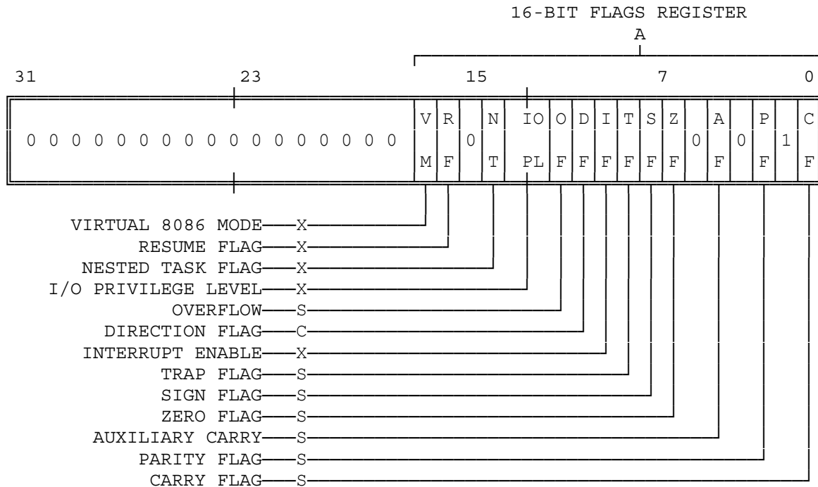
Figure 2-8. EFLAGS Register
