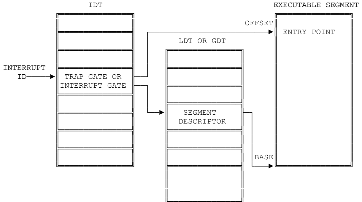
Figure 9-4. Interrupt Vectoring for Procedures
