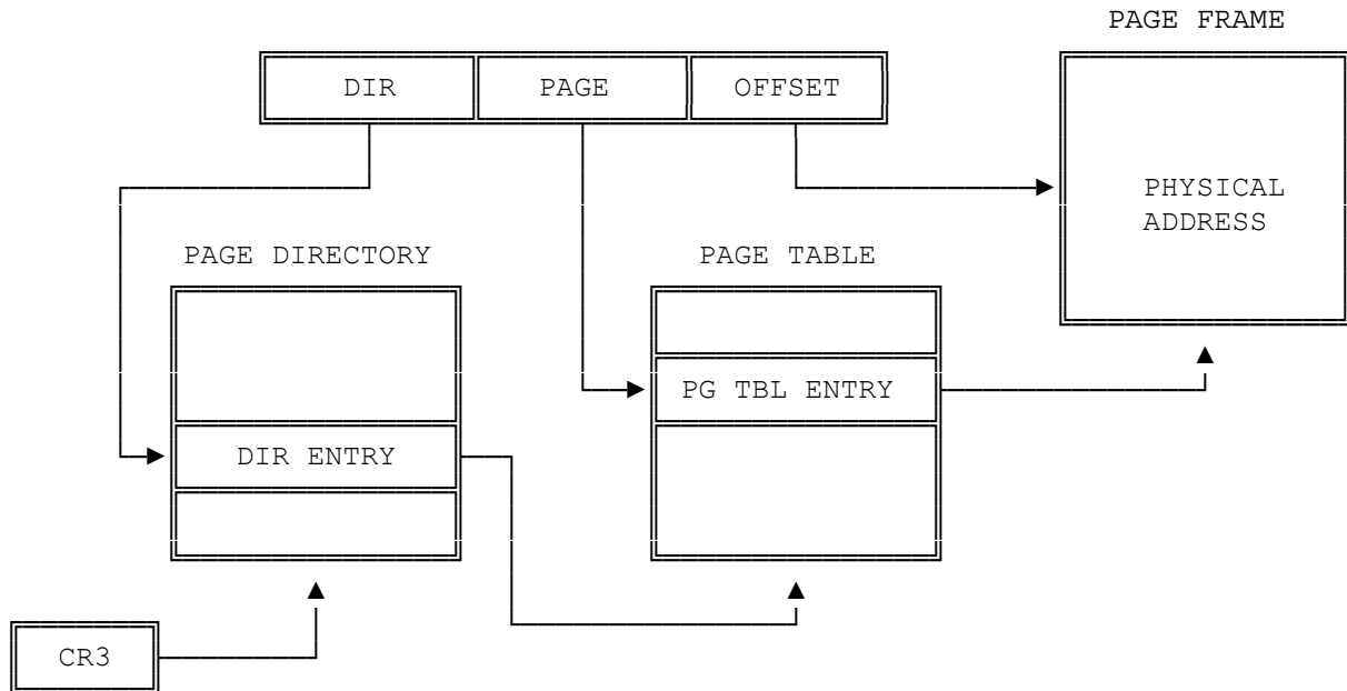
Figure 5-9. Page Translation
