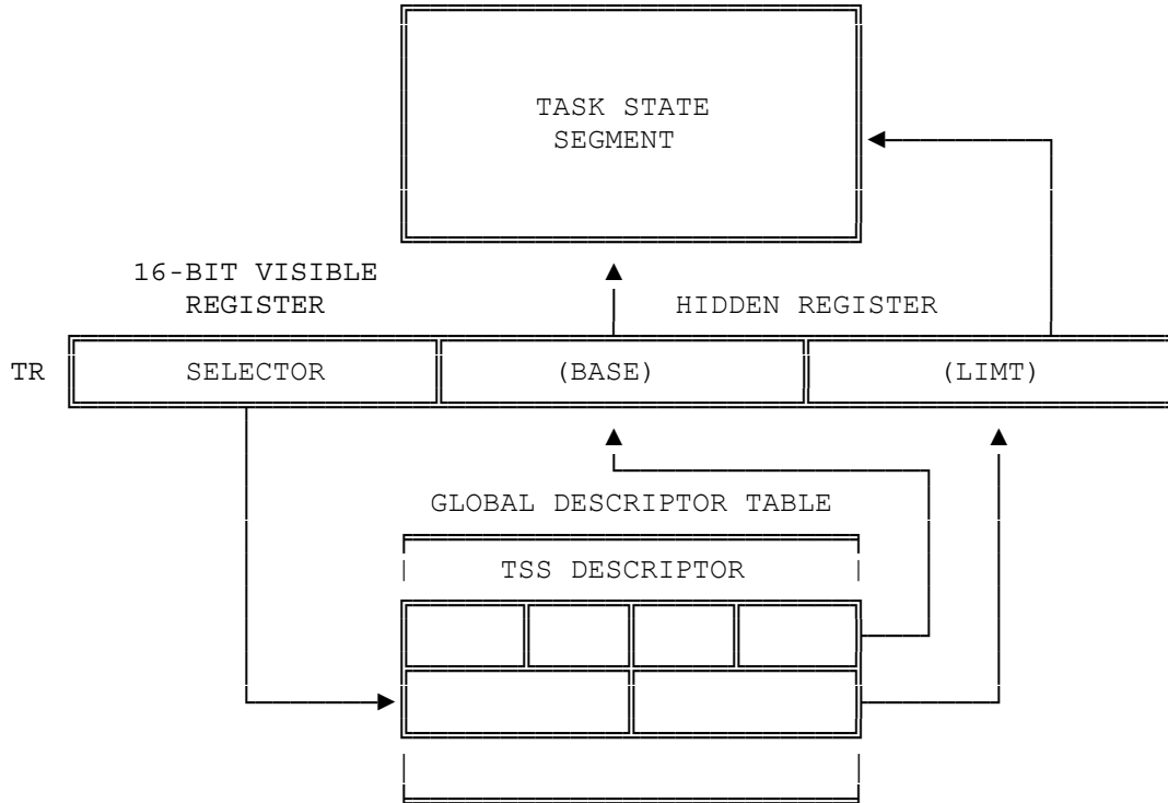
Figure 7-3. Task Register
