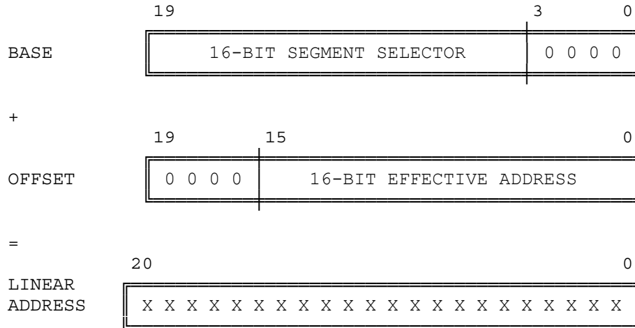
Figure 15-1. V86 Mode Address Formation
