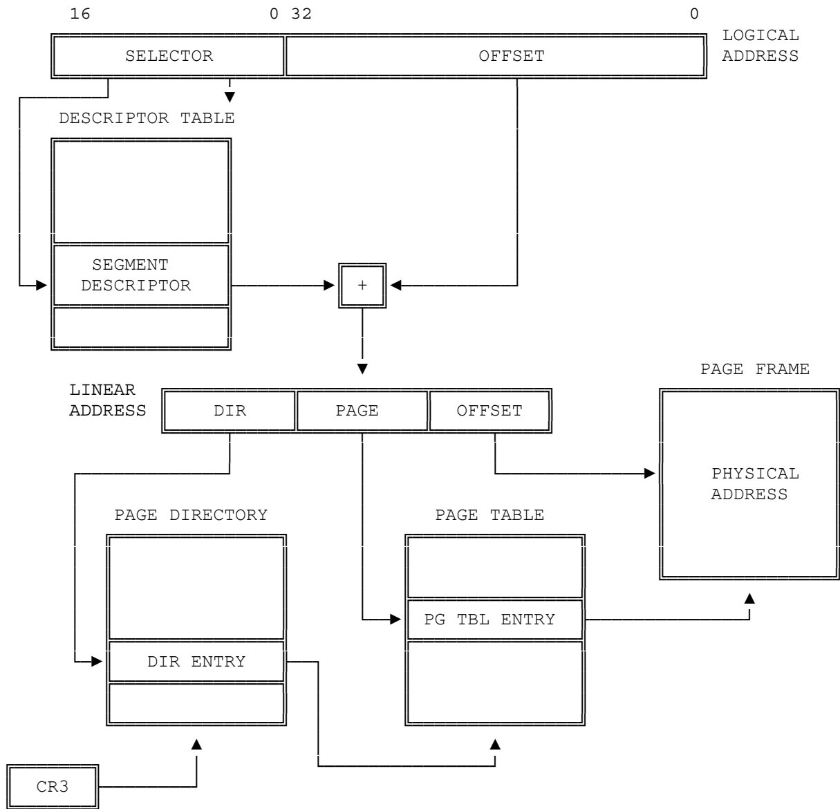
Figure 5-12. 80386 Addressing Mechanism
