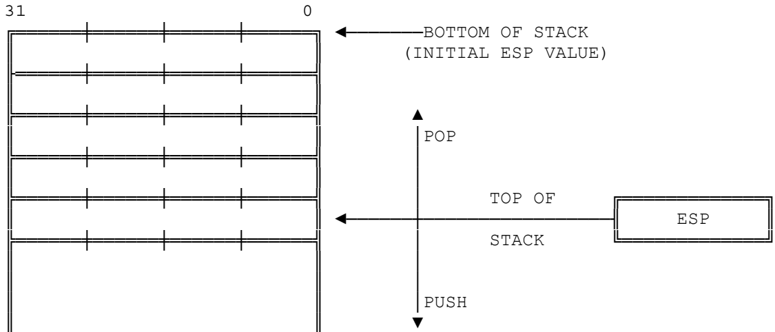
Figure 2-7. 80386 Stack
