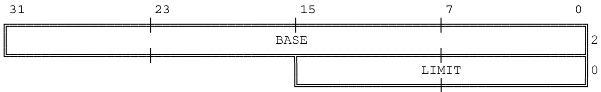
Figure 9-2. Pseudo-Descriptor Format for LIDT and SIDT
