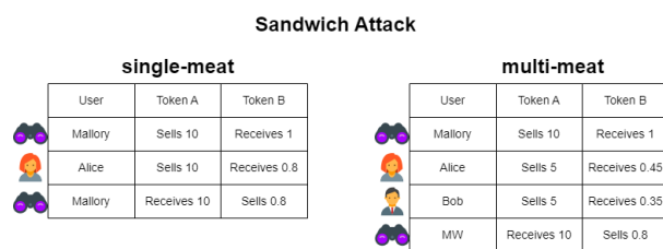
Fig. 7: Single versus multi-meat attacks.
