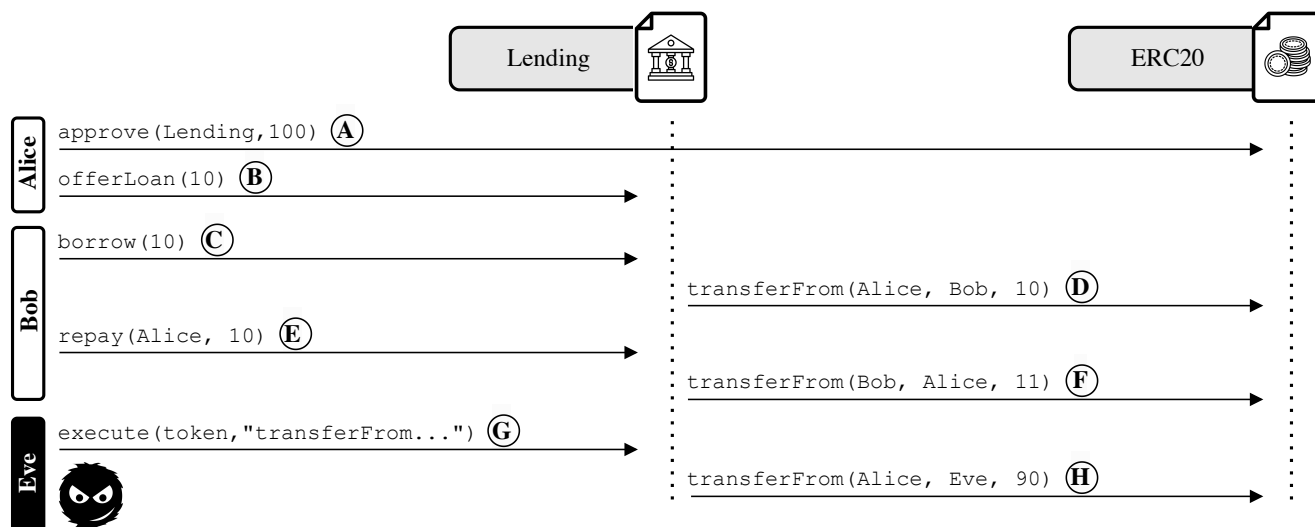
Figure 3: Simplified interaction flow of the Lending contract. Alice approves the Lending platform to manage 100 of her ERC20 tokens (A). Then, she lends 10 of her tokens (B). Bob requests to borrow 10 tokens (C). The Lending contract matches Bob’s request with a valid lender (Alice) and transfers 10 tokens from Alice to Bob (D). Later, Bob repays his debt – plus an interest fee (E/F). Eve notices that the execute function has improper access control, and calls it (G). The Lending contract executes Eve’s request and transfers 90 tokens from Alice to Eve (H).
