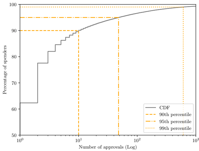
Figure 6: Cumulative distribution of number of approvals (log) among spenders (percentage).
