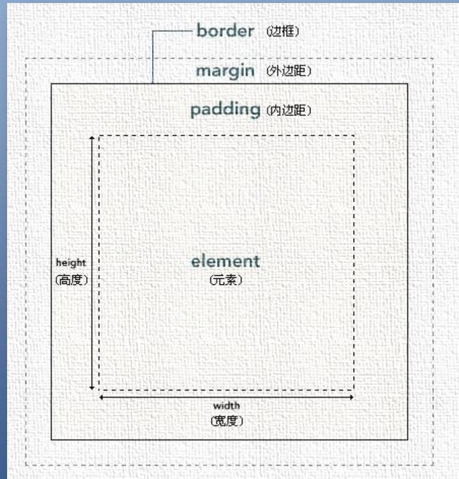
CSS Box Model
