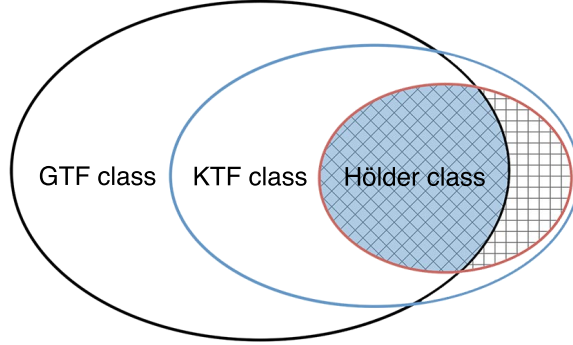
Figure 2: Illustration of the two higher-order TV classes, namely the GTF and KTF classes, as they relate to the (discretized) Holder class. The horizontally/vertically checkered region denotes the part of Holder class not contained in the GTF class. As explained in Section 4, this is due to the fact that the GTF operator penalizes discrete derivatives on the boundary of the grid graph. The diagonally checkered region (also colored in blue) denotes the part of the Holder class contained in the GTF class. The minimax lower bound rates we derive for the GTF class in Theorem 5 match the well-known Holder rates, suggesting that this region is actually sizeable and contains the “hardest” Holder smooth signals.
